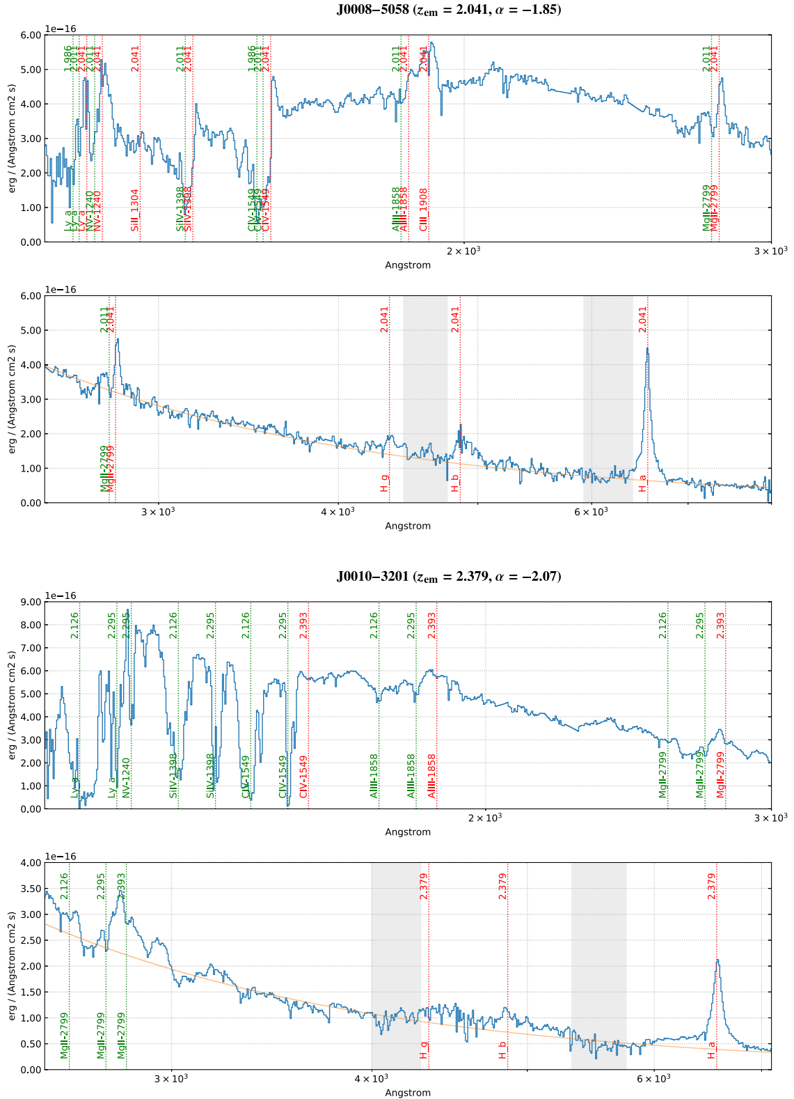
Figure 7. Spectra of other QUIP and non-QUIP QSOs from our sample. The legend is the same as in Fig. 6.
