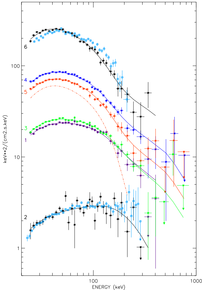
Figure 2. Evolution of the spectral shape of V404 Cyg on the 1–4 hr (labels 1–5) and 100 s (label 6) timescales. Crosses correspond to SPI data, and open squares to IBIS/ISGR data (for labels 2 and 6 only). Solid lines are the best common fit models, given in Table 1. See the text for the period definition.
