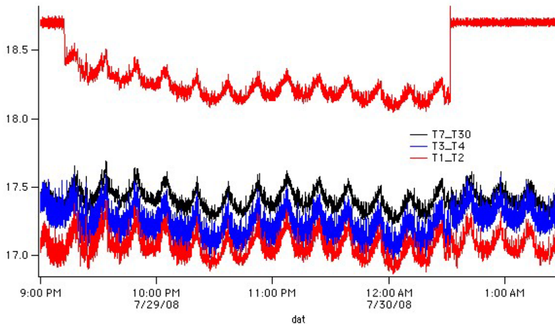
Figure 5-7-1. TSA shutoff.
