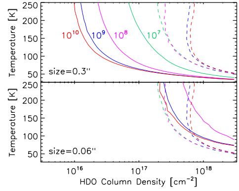
Fig. 4. LVG predictions of the temperature versus HDO column density required to reproduce the observed velocity-integrated emission (solid curves) and to have unit line opacity (dashed curves) for densities of: 10^7 cm ^{-3} (green), 10^8 cm ^{-3} (magenta), 10^9 cm ^{-3} (blue), and 10^{10} cm ^{-3} (red). Optical depth increases with column density. The upper panel refers to a source size of 0''.3 and the lower panel to 0''.06 .
