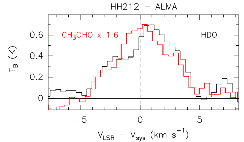
Fig. 3. Comparison between HDO( 33_{1,1} – 42_{2,2} ) (black line) and CH 3 CHO( 18_{0,18} – 17_{0,17} )A (red, multiplied by a factor of 1.6) as observed towards HH212–MM1 (in T_B , scale). The vertical dashed line defines the velocity with respect to V_{\text{sys}} = +1.7 km s ^{-1} (see footnote 2).
