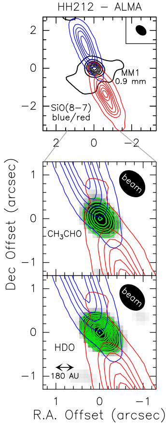
Fig. 1. Upper panel: The HH212 protostellar system as observed by ALMA–Band 7 (Codella et al. 2014). Blue/red contours plot the blue-/redshifted SiO(8–7) jet at \pm 8 km s ^{-1} from V_{\text{sys}} , overlaid on the 0.9 mm continuum (black contours). Positions are with respect to the coordinates reported in Sect. 2. The filled ellipse shows the synthesised beam (HPBW) for SiO: 0''.63 \times 0''.46 (PA = 49^\circ ). Middle panel: Zoom-in of the central region: the CH 3 CHO( 18_{0,18} – 17_{0,17} )A emission integrated over \pm 5 km s ^{-1} (green contours and grey scale) overlaid on the SiO jet. First contours and steps are 5\sigma (50 mJy beam ^{-1} km s ^{-1} ) and 2\sigma , respectively. The HPBW is 0''.69 \times 0''.52 (PA = 42^\circ ). Bottom panel: Same as middle panel for HDO. The HPBW is 0''.68 \times 0''.51 (PA = 42^\circ ).
