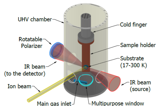
Figure 1: Schematic view of the experimental set-up.
