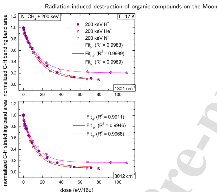
Figure 3: Normalized C-H bending and C-H stretching band area of N 2 :CH 4 mixtures after ion bombardment plotted vs. irradiation dose. The graphs show data resulting from the irradiation with H + , He + and N + 200 keV ions and the fit obtained using Eq. 1.
