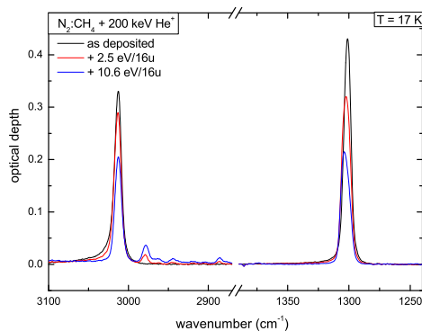
Figure 2: Evolution of C-H stretching and bending peaks a for \text{N}_2:\text{CH}_4 mixture after ion irradiation: the initial stage is represented in black, and two steps of irradiation in red and blue.
