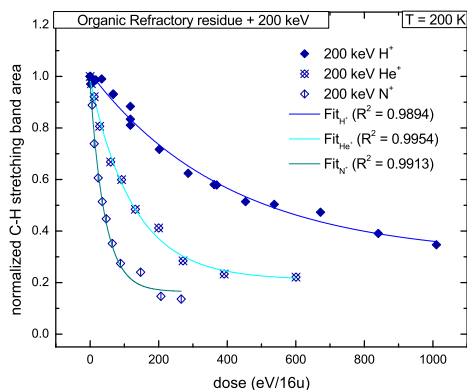
Figure 8: Normalized C-H stretching band area of the organic refractory residue after ion bombardment plotted vs. irradiation dose. The graph shows data obtained from the irradiation with 200 keV H^+ , He^+ and N^+ and the fit obtained using Eq. 1.
