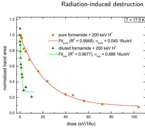
Figure 6: Normalized band area of pure and diluted formamide after ion bombardment plotted vs. irradiation dose. The graph shows data resulting from the irradiation with H^+ 200 keV ions and the fit obtained using Eq. 1.
