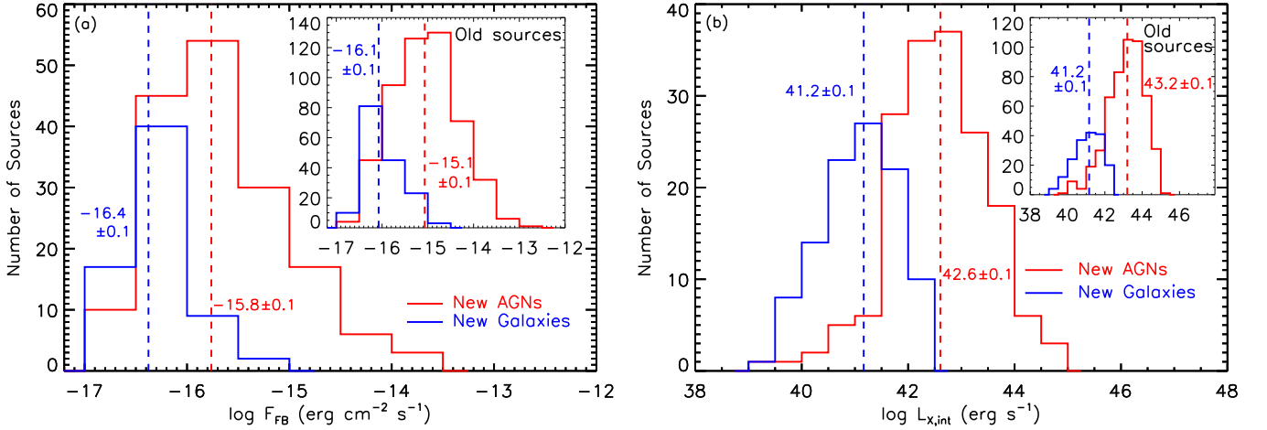
Figure 25. Distributions of (a) full-band fluxes and (b) intrinsic 0.5–7.0 keV luminosities for the newly detected main-catalog sources. In each panel, the inset displays the corresponding distributions for the main-catalog sources that were present in the Xue et al. (2011) 4 Ms CDF-S catalogs. The red and blue histograms indicate the distributions for AGNs and galaxies, respectively. The vertical dashed lines show the median values of the corresponding distributions, and the numbers display the corresponding median values and their 1\sigma uncertainties (derived via bootstrapping). Sources with upper limits on the full-band fluxes (92 sources; 9%) are not included in panel (a). The 22 sources that lack redshifts and the 12 stars are not included in panel (b).
