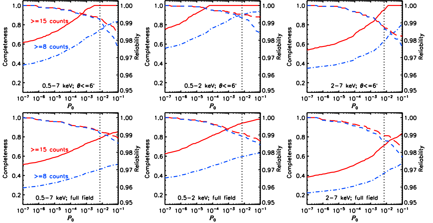
Figure 27. Completeness (left y-axis; solid and dash-dotted curves) and reliability (right y-axis; long-dashed and short-dashed curves) as a function of the P_B threshold value, P_0 , for sources with \geq 15 counts (red solid and long-dashed curves) and \geq 8 counts (blue dash-dotted and short-dashed curves) in the full, soft, and hard bands, respectively. The top panels show the completeness and reliability curves for the central 6'-radius region and the bottom panels show those for the entire CDF-S field. The vertical dotted lines indicate our adopted main-catalog P_B threshold of 0.007.
