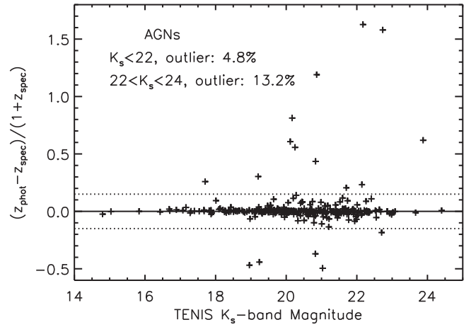
Figure 11. Photometric redshift accuracy vs. TENIS K_s -band magnitude for the AGNs in the main catalog that have photometric redshifts from Hsu et al. (2014) and also secure spectroscopic redshifts. The solid and dashed lines indicate (z_{\text{phot}} - z_{\text{spec}})/(1 + z_{\text{spec}}) values of 0, 0.15, and -0.15 , respectively. The outlier fraction of the photometric redshifts increases toward larger K_s -band magnitudes.
