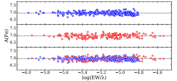
Fig. 2. Iron abundances as a function of the reduced EW for all the measured optical (blue circles) lines in the UVES spectra and NIR (red circles) lines in the GIANO-B spectrum. The dotted line marks the best-fit median abundance.
