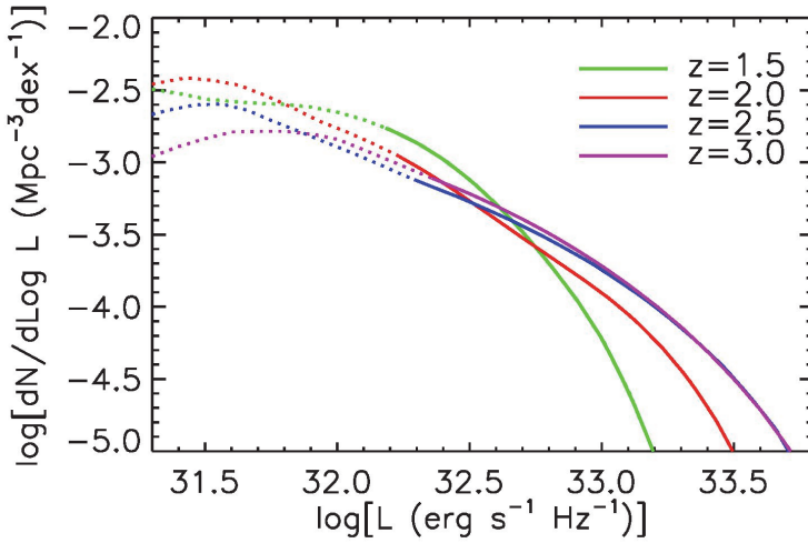
Fig. 3. Portions of the 500 \mu m galaxy luminosity function at various z covered by Herschel surveys to a flux limit of 50 mJy. The corresponding fraction of resolved luminosity density ranges from 29% to 66%.
