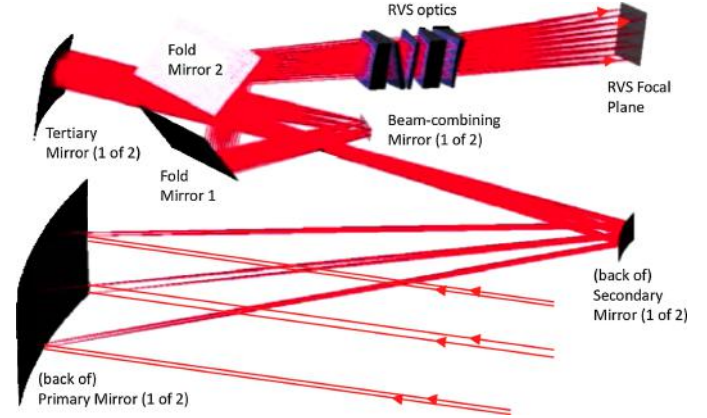
Fig. 2. RVS optical path for one telescope. The primary mirror is at the lower left, and the RVS focal plane at the upper right, with the RVS optics immediately preceding it in the light path. Below the RVS optics is one half of the beam-combining mirror.
