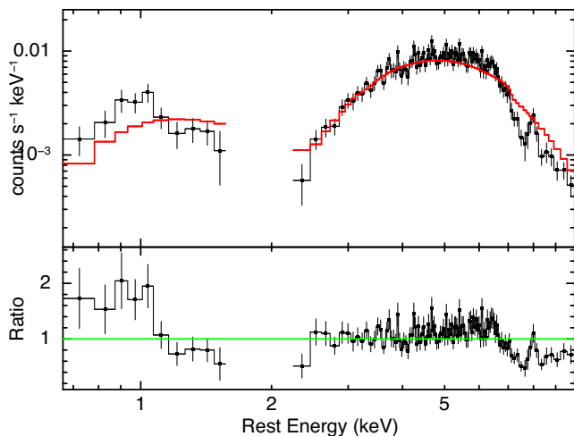
Figure 1. The upper panel shows the XIS-FI data (black data points) and a simple continuum model (shown in red), which is composed of an absorbed power-law component ( \Gamma = 2 , N_H \sim 2.5 \times 10^{23} \text{ cm}^{-2} ) and a scattered soft power-law component. The lower panel shows the data/model ratio to this model. Clear residuals are visible in the soft X-ray band, due to possible thermal emission, and at the iron K-shell energy band. Besides a weak Fe K \alpha emission line at \sim 6.4 keV, two strong absorption features are apparent at \sim 7.4 and \sim 8.5 keV.
