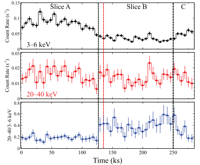
Figure 5. NuSTAR light curves extracted (with a bin size of 5814 s) in the 3–6 keV (upper panel) and the 20–40 keV band (middle panel). The lower panel shows the hardness ratios (HR) light curve defined as \text{CR}_{20-40 \text{ keV}} / \text{CR}_{3-6 \text{ keV}} . While there are only small fluctuations in the 20–40 keV light curve, the 3–6 keV light curve presents a sharp drop at around 125 ks (marked with the black dashed line) into the observation and a smooth increase at the end of the observation (at around 250 ks, black dashed line). The HR light curve (lower panel) shows a sharp increase at 125 ks, suggesting that we are witnessing an obscuration event. At 250 ks the HR starts to decrease to almost the initial value. The red dashed line marks the end of the XMM-Newton observation at around 140 ks.
