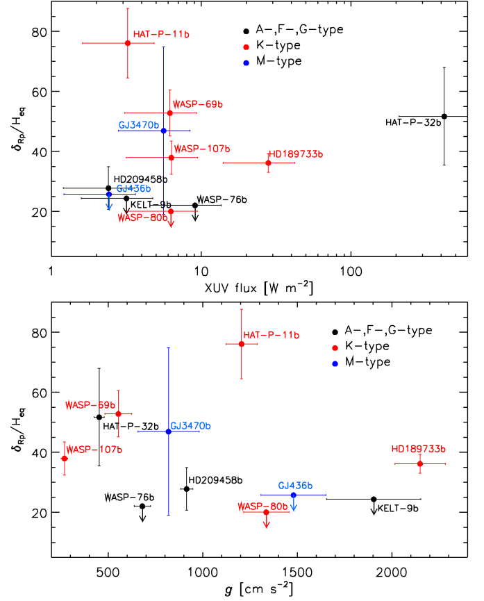
Fig. B.1. Top: size of the measured HeI absorption signal, normalised to the atmospheric scale height computed considering the planetary parameters listed in Table 3 and a mean molecular weight of a pure hydrogen atmosphere, as a function of the incident stellar XUV flux (in logarithmic scale). Upper limits are marked by downward arrows. The symbol color indicates the spectral type of the host as given by the legend. Bottom: as the upper panel, but as a function of planetary surface gravity.
