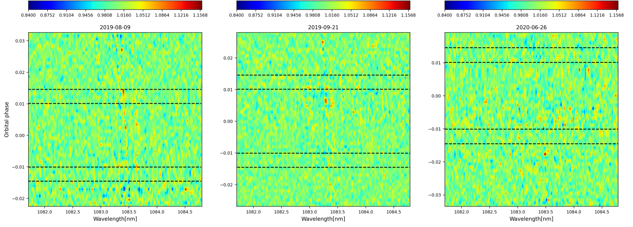
Fig. A.1. Transmission spectra shown in tomography in the planetary rest frame for the three considered transits, as a function of wavelength and planetary orbital phase. The contact points t_1 , t_2 , t_3 , and t_4 are marked with horizontal black lines. The feature at 1083.5 nm misaligned with the planet rest frame present in the first and second night is a residual of a telluric \text{H}_2\text{O} line.
