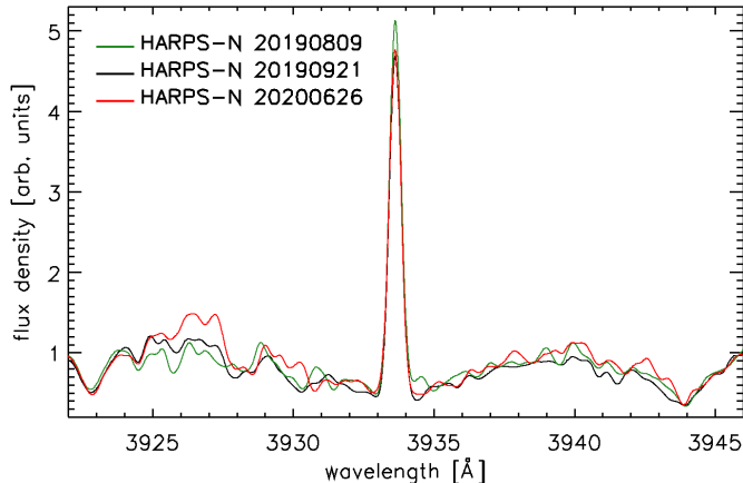
Fig. 5. Comparison among the master HARPS spectra of the CaII K line obtained combining the data collected within each night and convolved to a spectral resolution of 10,000, for visualisation purposes.
