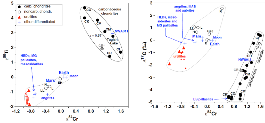
Fig. 2 Dichotomy of stable isotopes among planetary materials. (Figure reprinted from Warren, 2011).
