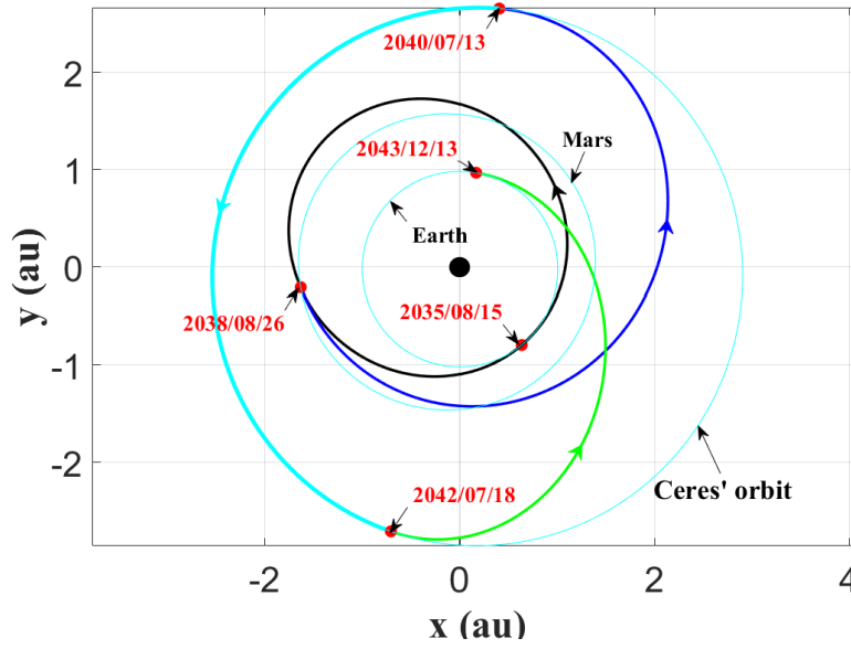
Fig. 10 The transfer trajectory for Ceres' sample return mission. In the transfer scenario, a Mars gravity assist is taken into consideration in order to save fuel consumption. The probe launches on August 15 th, 2035. The arc from the Earth to Mars is shown in black line; the arc from Mars to Ceres is given in blue line; the rendezvous segment is presented in cyan; and the return trajectory from Ceres to the Earth is marked in green. The key points of time are represented by red dots.
