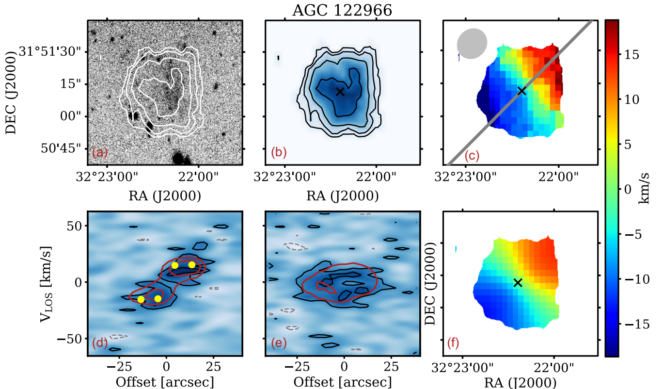
Figure A1. VLA data and kinematic models for AGC 122966. Panels and symbols as in Fig. 1. The H I contours are at 0.5, 1, 2 and 4 × 10 20 atoms cm -2 .
