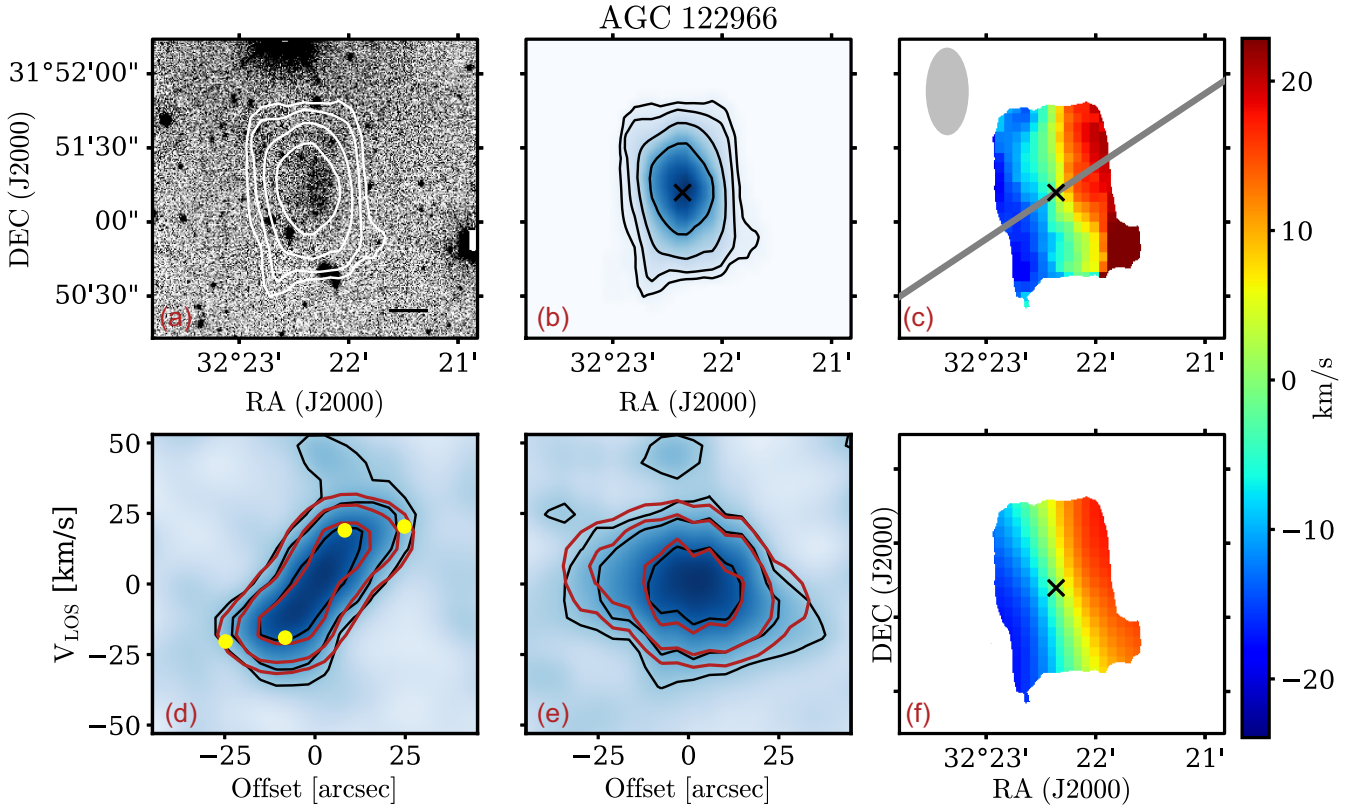
Figure 2. Data and kinematic models for the gas-rich UDG AGC 122966. Panels and symbols as in Fig. 1. The H I contours are at 0.35, 0.7, 1.4 , and 2.8 \times 10^{20} atoms \text{cm}^{-2} . Note that the kinematic and morphological position angles seem to be different, but this apparent effect is due to the peculiar elongated shape of the WSRT beam (see Appendix A).
