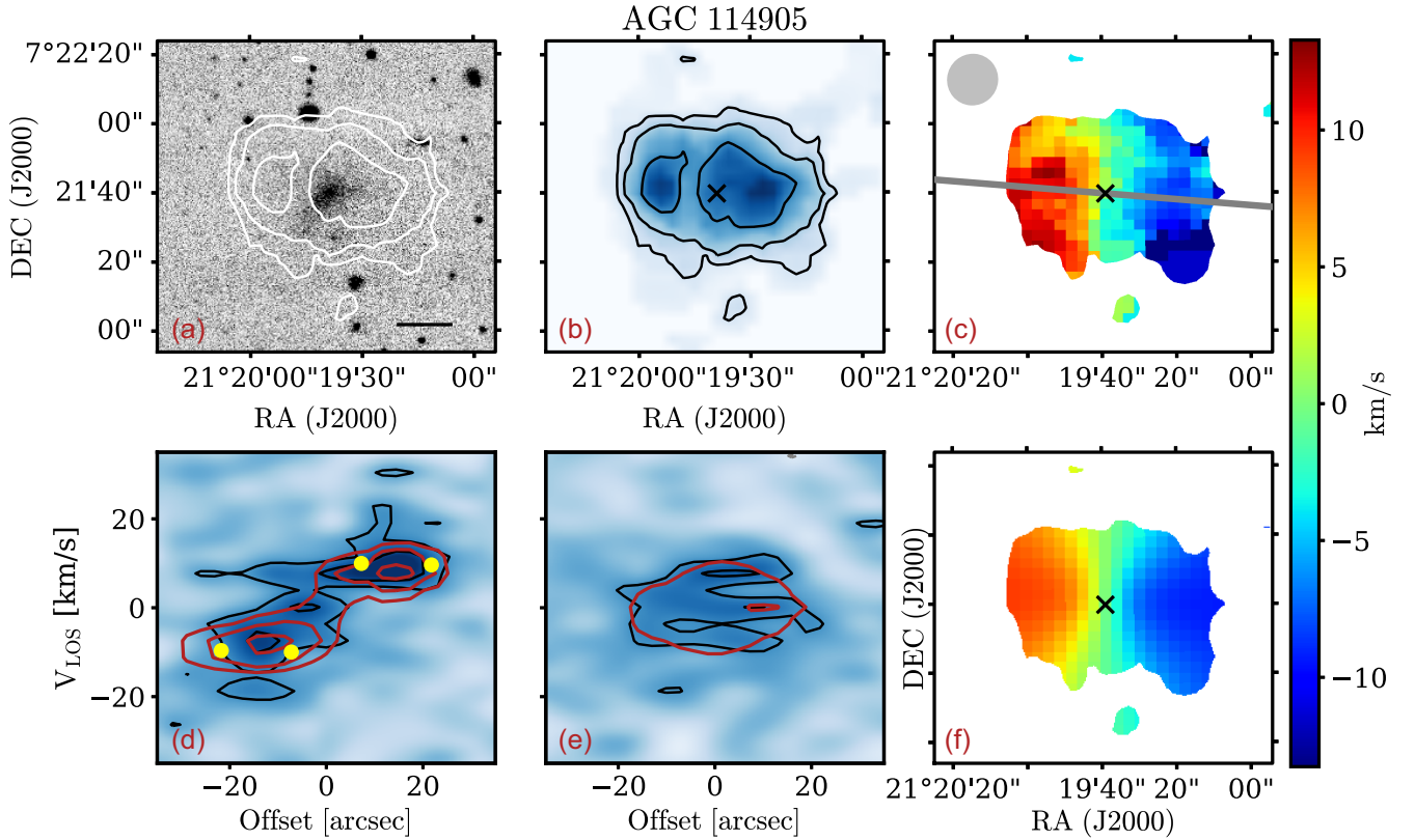
Figure 1. Data and kinematic models for the gas-rich UDG AGC 114905. (a) r – band image with H I contours on top at 1, 2 , and 4 \times 10^{20} atoms \text{cm}^{-2} , with the lowest one at S/N \approx 3 . The black solid line indicates a physical scale of 5 kpc. (b) Total H I map in blue, and contours as in panel (a). (c) Observed velocity field (first-moment map). The grey line shows the major axis, while the grey ellipse shows the beam. (d) PV diagram along the major axis. Black and red contours correspond to data and best-fitting model, respectively, and are at the 2\sigma and 4\sigma levels. If present, grey dashed contours indicate negative values in the data. The recovered rotation velocities are indicated with the yellow points. (e) PV diagram along the minor axis (perpendicular to the major axis), colours as in (d). (f) Modelled velocity field. The black cross in panels (b), (c), and (f) shows the kinematic centre. The rightmost panel shows the velocity colour bar for panels (c) and (f).
