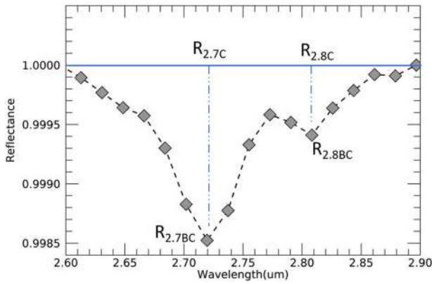
Fig. 2. The 2.7- \mu\text{m} and 2.8- \mu\text{m} isolated bands, after the removal of the unique continuum (represented by the blue line). The NIRS3 spectral bands are the grey diamonds and values of reflectance useful for the estimation of band depths are marked. (For interpretation of the references to colour in this figure legend, the reader is referred to the web version of this article.)
