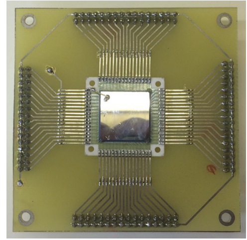
Fig. 2. The cathode view of the ACRORAD 8 \times 8 CdTe detector inside a metallic shielded box that was closed by a metal cover with an entrance window of 20 mm diameter and 20 \mu\text{m} thick Al foil.
