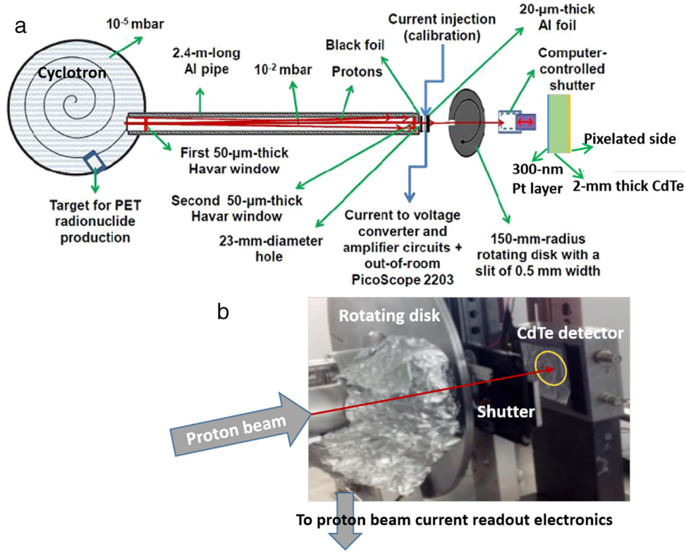
Fig. 3. (a) Schematic view of ICNAS cyclotron proton irradiation and mechanical setup to collimate and tune the proton beam onto the CdTe matrices. The protons dispersion in the first 50 \mu m thick Havar window is illustrated by the indicated paths, justifying the lateral straggling of the proton beam at the outlet of the aluminum tube. (b) Detail of the last stage of the proton irradiation setup [21].
