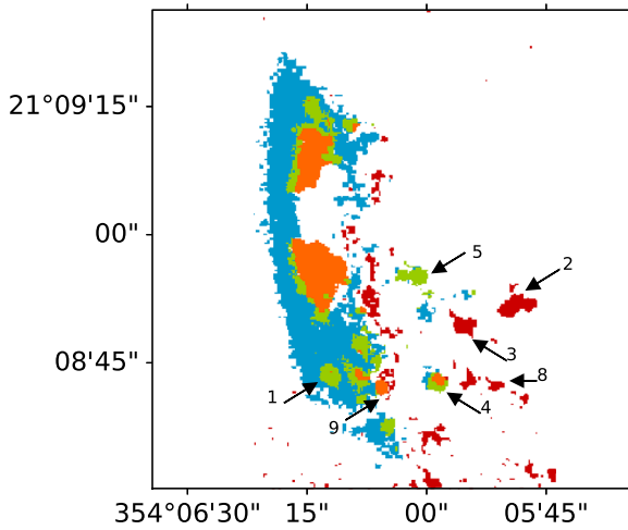
Figure 8. The SF sequence created by ram pressure: only CO (red), CO+SF-powered H \alpha +UV (orange), SF-powered H \alpha +UV (green), and only UV (cyan). The regions with SF-powered H \alpha are also star-forming according to the [O I] line (right panel in Figure 2). Numbers are the same as in the middle left panel of Figure 7.
