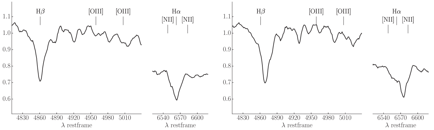
Figure 9. Spectra of regions (6) (left) and (7) (right); see red squares in Figure 7.
