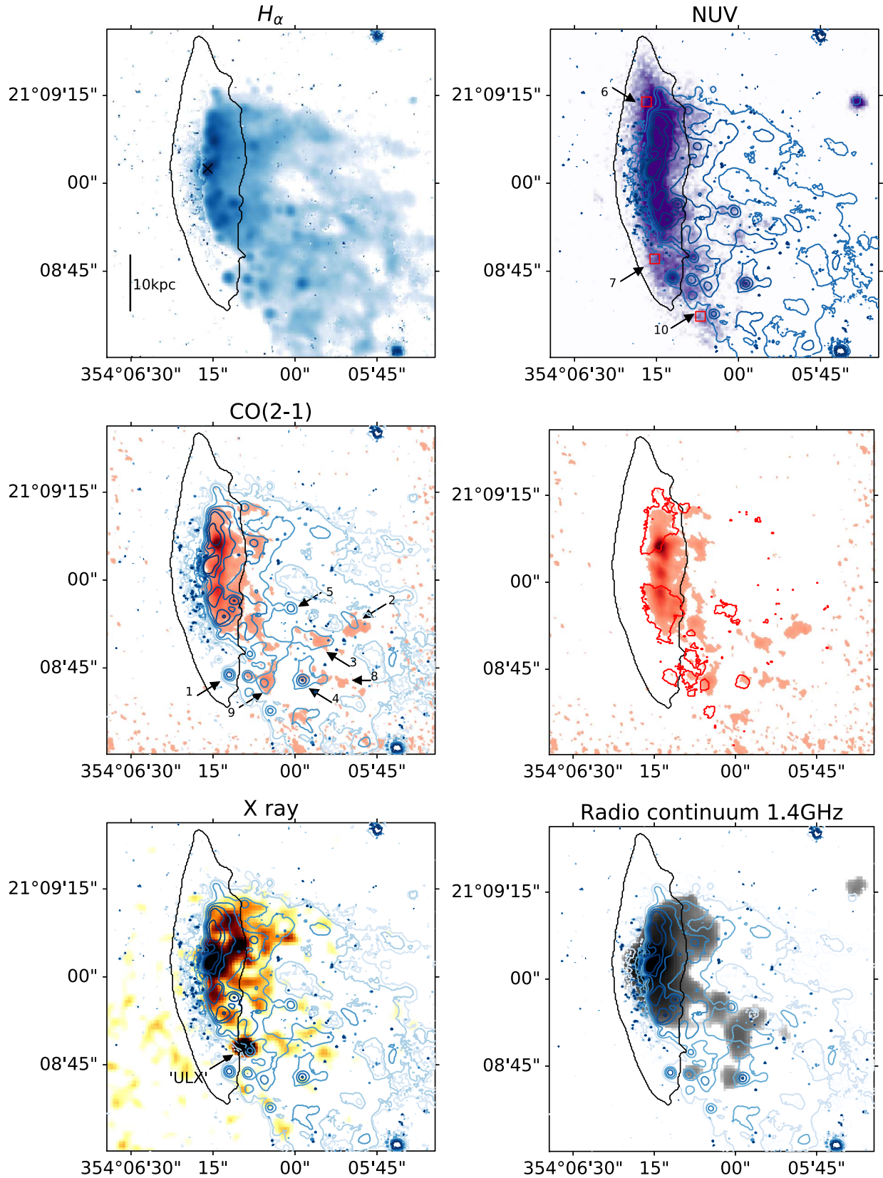
Figure 7. The JW100 multiwavelength tails. Images displayed are (top panels) the MUSE H_\alpha ( 1'' resolution) and UVIT NUV ( 1''/2 ), (middle) ALMA CO(2–1) ( 1'' ), and (bottom) Chandra X-ray ( 0''/5 ) and VLA 1.4 GHz ( 3''/8 \times 3''/4 ). Overlaid blue contours are the MUSE H_\alpha emission. The red contours in the middle right panel outline the star-forming regions in Figure 2. The stellar disk region is shown by the black contours. The positions marked with arrows and numbers are discussed in the text (Section 4.1). The cross in the top left panel identifies the galaxy center, defined as the centroid of the continuum (stellar) emission underlying the H_\alpha line from MUSE.
