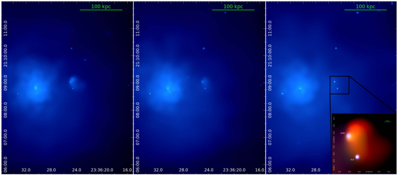
Figure 4. Cluster-scale images showing the three X-ray bands (soft 0.5–1.2 (left), medium 1.2–2.0 (middle), and hard 2.0–7.0 (right) keV) of the field of JW100, smoothed with csmooth in CIAO. The inset in the right panel is an RGB (red = 0.5–1.2, green = 1.2–2.0, and blue = 2.0–7.0 keV) smoothed zoom on the galaxy where the two point sources (AGN and ULX candidate) are clearly visible.
