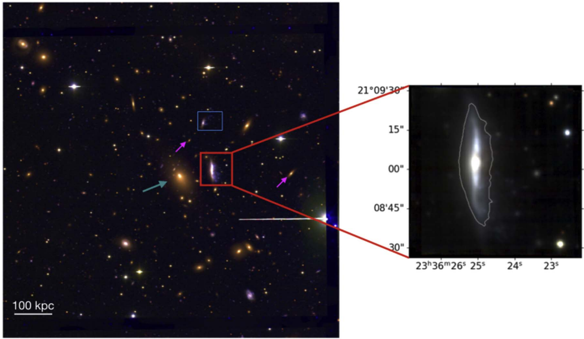
Figure 1. An RGB image of A2626 (NUV-B-V, UVIT+WINGS) and a zoomed-in image of JW100 ( gri MUSE). In the inset, the white contour represents the most external ( \sim 1.5\sigma above background) isophote of the continuum MUSE light under H\alpha and delineates the stellar disk. The major axis of this contour is 50 kpc. The green arrow points to the BCG, the pink arrows point to the other two galaxies belonging to the JW100 substructure (Section 2.1), and the blue rectangle identifies the other jellyfish, JW103.
