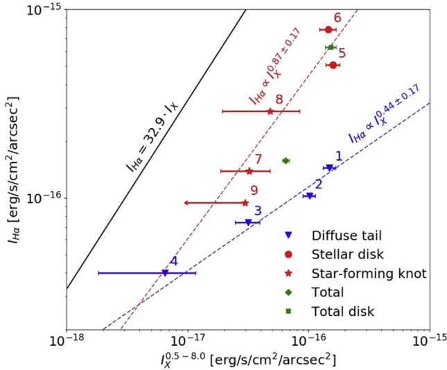
Figure 10. The H\alpha vs. 0.5–8 keV X-ray surface brightness in the different regions identified with yellow polygons in Figure 2. The blue triangles are the four regions of diffuse emission with LINER-like [O I]/ H\alpha ratios in the right panel of Figure 2. Red indicates the regions where the [O I]/ H\alpha ratio (as well as [S II]/ H\alpha ) indicates SF: the star-forming regions within the disk (circles) and the knots in the tail (stars). Green shows the total and disk values. The blue dashed line is the fit to the blue diffuse emission points. The solid black line is the expected relation combining the L_X = \text{SFR} relation from Mineo et al. (2014) and the L_{H\alpha} = \text{SFR} relation from Kennicutt (1998).
