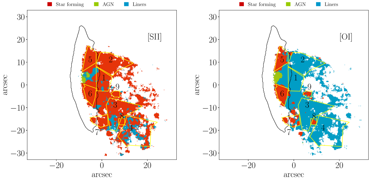
Figure 2. Ionization mechanism map according to (left) the [O III] 5007/H \beta vs. [S II] 6717,6731/H \alpha and (right) [O III] 5007/H \beta vs. [O I] 6300/H \alpha diagnostic diagrams. Red = SF, green = AGN, and blue = LINER-like emission. The yellow polygons define the regions that are studied in Section 5.3. The black contour shows the stellar disk as in Figure 1.
