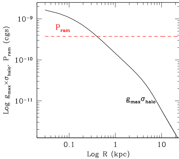
Figure 11. The ICM ram pressure (red dashed line) versus the component along the direction of motion of the restoring force per unit area (solid black line) for the fiducial model with the Miyamoto–Nagai disk.
