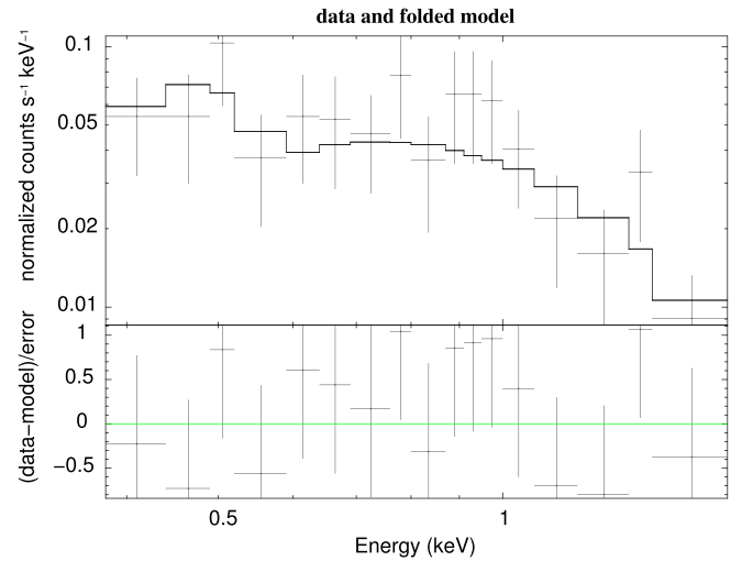
Figure 6. The 0.3–1.7 keV spectrum of SN 2015J as observed by Swift /XRT (OBs ID 00033857012).
