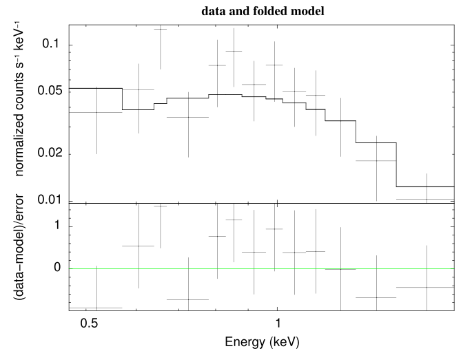
Figure 7. The 0.3–1.7 keV spectrum of SN 2015J as observed by Swift /XRT (OBs ID 00033857013).
