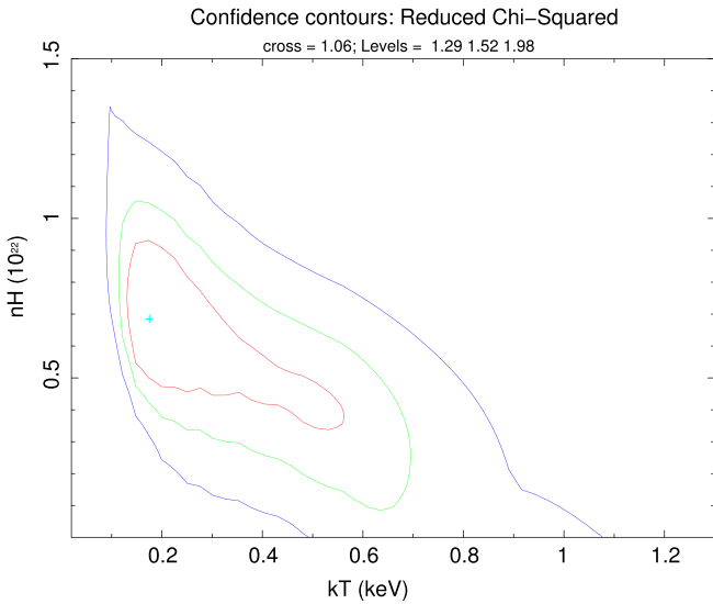
Figure 8. Contour plot of the temperature and absorption column parameters from a fit of an intrinsically absorbed MEKAL model to the Swift observation of 2017 July (assuming z = 0.0054 and a galactic column density nH = 2.0 \times 10^{21} \text{ cm}^{-2} ). The contours mark the 1\sigma , 2\sigma and 3\sigma errors.
