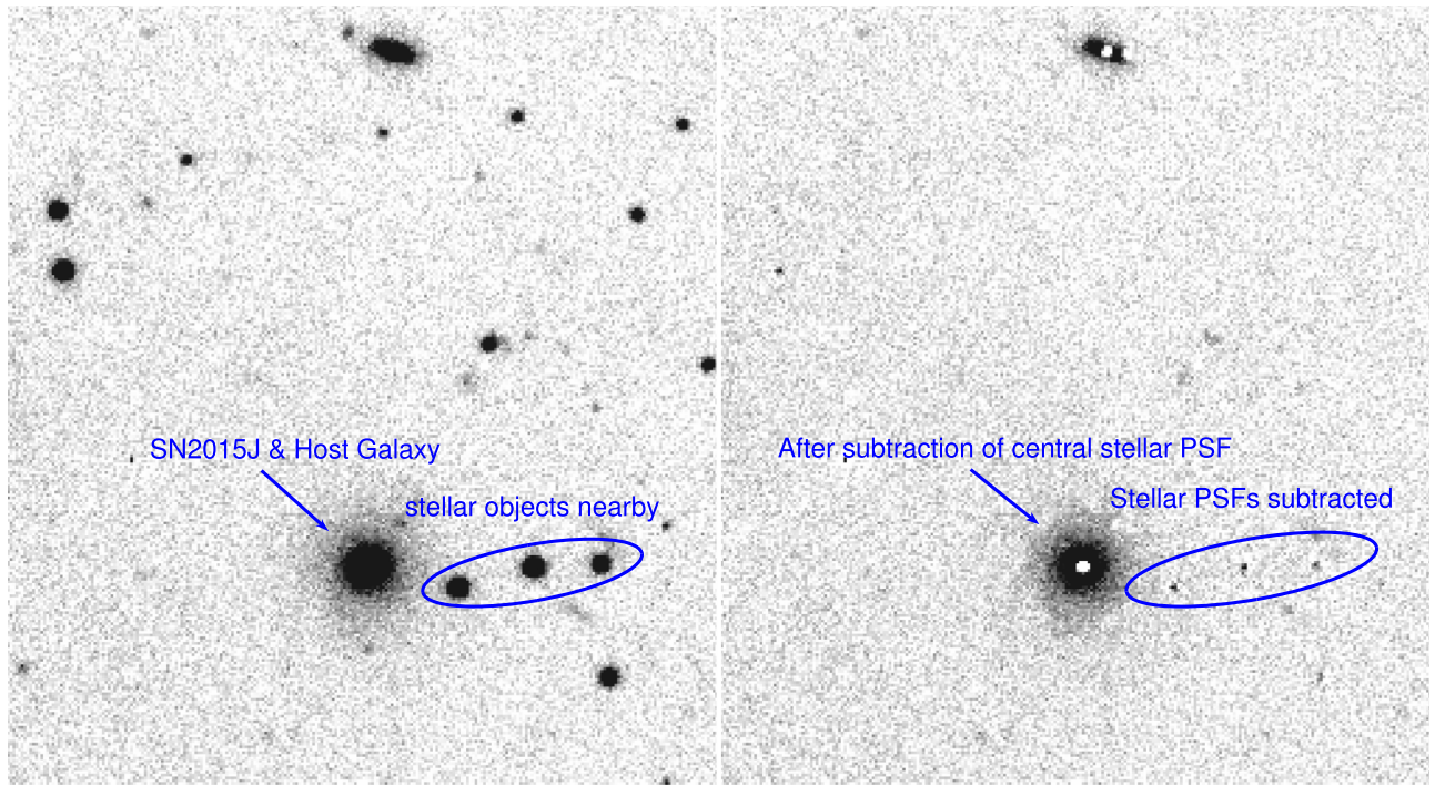
Figure 2. The VLT/FORS2 image of the region around SN 2015J before (left panel) and after (right panel) subtracting the PSF obtained using DAOPHOT. As can be seen, the target source is an extended object, probably a dwarf galaxy (see the text for details).
