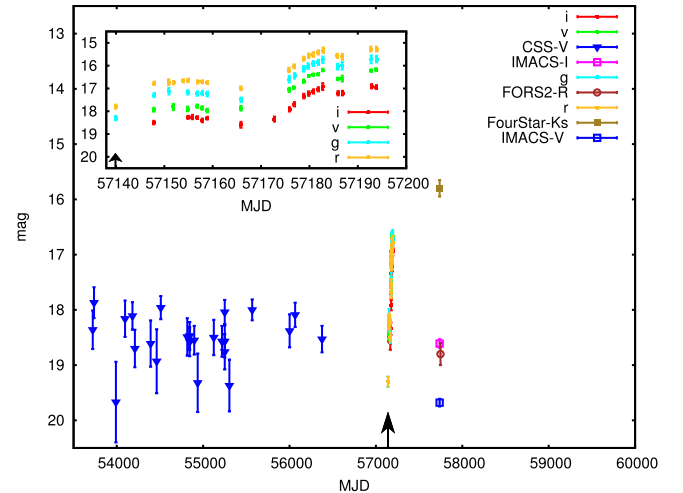
Figure 4. The multi-band light curve of the target, including the CSS data (filled triangles; see the text for details), is shown. The inset shows a zoom-in of the light curve (dots as taken directly from Childress et al. 2015) about the time of the SN event that occurred on 2015 April 27.9 UT (corresponding to MJD = 57139.9, as also indicated by the black arrow). From the i band to the r band we applied a recursive offset of 0.5 mag for each light curve shown in the inset. The data used to create this figure are available.
