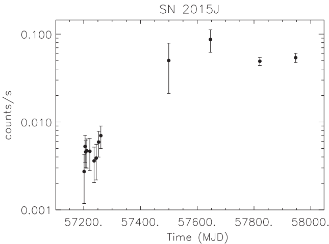
Figure 5. The 0.3–10 keV light curve of SN 2015J. The last data point (acquired by SWIFT /XRT in 2017 July) shows that the SN event is still active in the X-rays after more than one year at a level of \approx 0.05 counts s -1 . The XMM slew flux at MJD = 57646.5 has been converted into a Swift count rate (see the text for details).
