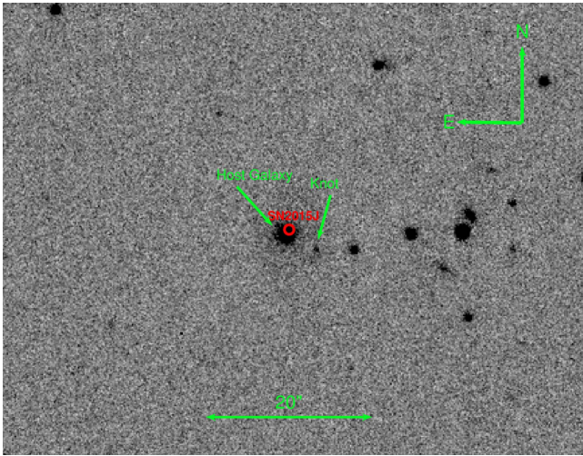
Figure 3. The FourStar Ks image of the galaxy host of SN 2015J.
