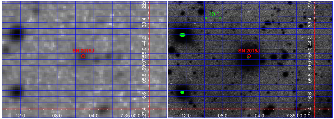
Figure 1. The DSS F_{ph} band image (left panel) and the image acquired by the VLT/FORS2 in the R band (right panel) of the region toward SN 2015J are shown. The red circle is centered on SN 2015J. The green circle (with a 0''.5 radius and centered on the centroid of the corresponding brightness surface) appearing in the right panel corresponds to the source detected in the VLT/FORS2 image.
