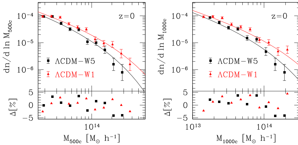
Figure 15. SOD halo mass functions from \Lambda CDM-W5 (black squares) and \Lambda CDM-W1 (red triangles) with mass M_{500c} (left panel) and M_{1000c} (right panel), respectively, against the ST-RayGal predictions.
