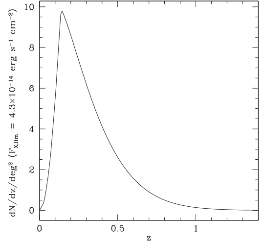
Figure 12. Expected redshift distribution of clusters of an eROSITA -like survey with X-ray flux cut F_{X,\text{cut}} = 4.3 \times 10^{-14} \text{ erg s}^{-1} \text{ cm}^{-2} for our fiducial cosmological model.
