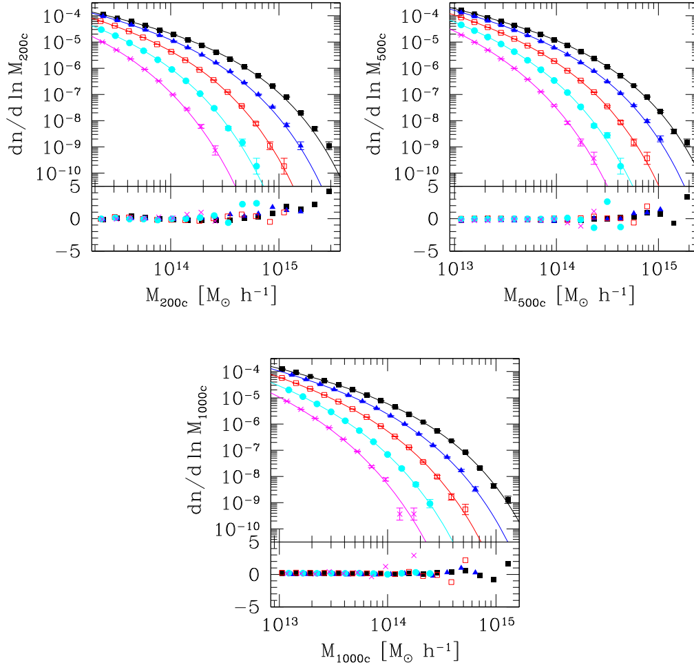
Figure 14. Halo mass function from the RayGalGroupSims simulation for SOD halos with mass M_{200c} (top left panel), M_{500c} (top right panel), and M_{1000c} (bottom panel) at z = 0, 0.5, 1, 1.5 , and 2 (top to bottom). The solid lines are the ST-RayGal mass functions with coefficients given by Equations (15), (16), and (17). The logarithmic residual is shown in the bottom panel: as we can see, deviations are within the 5% level across the entire mass range.
