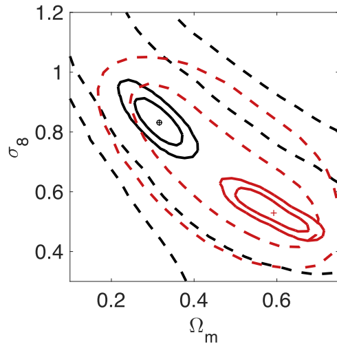
Figure 6. 1\sigma and 2\sigma credibility contours in the \Omega_m – \sigma_8 plane from the likelihood analysis of average sparsity data with 1% (solid lines) and 20% (dashed lines) statistical errors generated by solving Equation (4) with the ST-RayGal mass function. The black lines correspond to the constraints shown in Figure 5 inferred assuming the ST-RayGal mass function. The constraints obtained assuming the ST-Despali mass function are shown as red lines. The black circle indicates the fiducial model parameters, while the plus signs indicate the best-fit parameter values for the different parameterizations.
