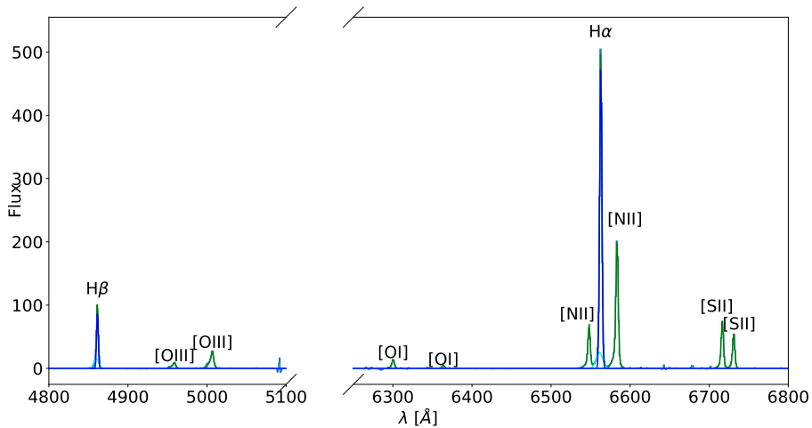
(d) Integrated spectrum: The spectrum is shown in light blue, the two-component fit in green, the one component fit in dark blue and for the broad components of Hα and Hβ in cyan.
