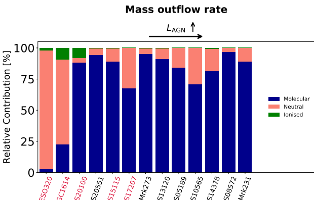
Figure 5. Relative contribution of the molecular (blue), ionized (green) and neutral atomic (red) phases to the total mass outflow rate. The galaxies whose names are in red are star forming galaxies. The galaxies are sorted by increasing AGN luminosity from left to right.
