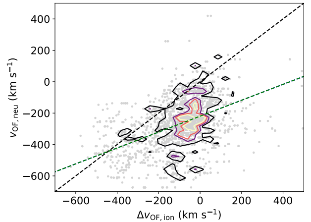
Figure 9. Neutral outflow velocity ( v_{50} ) versus ionized outflow blueshift for all spaxels of all galaxies. The coloured isodensity contours correspond to 10, 30, 50 and 70 points in that bin (the parameter space has been divided into 50 bins). The dashed black line indicates the 1:1 correlation, the green dashed line is the best fit to the data points.
