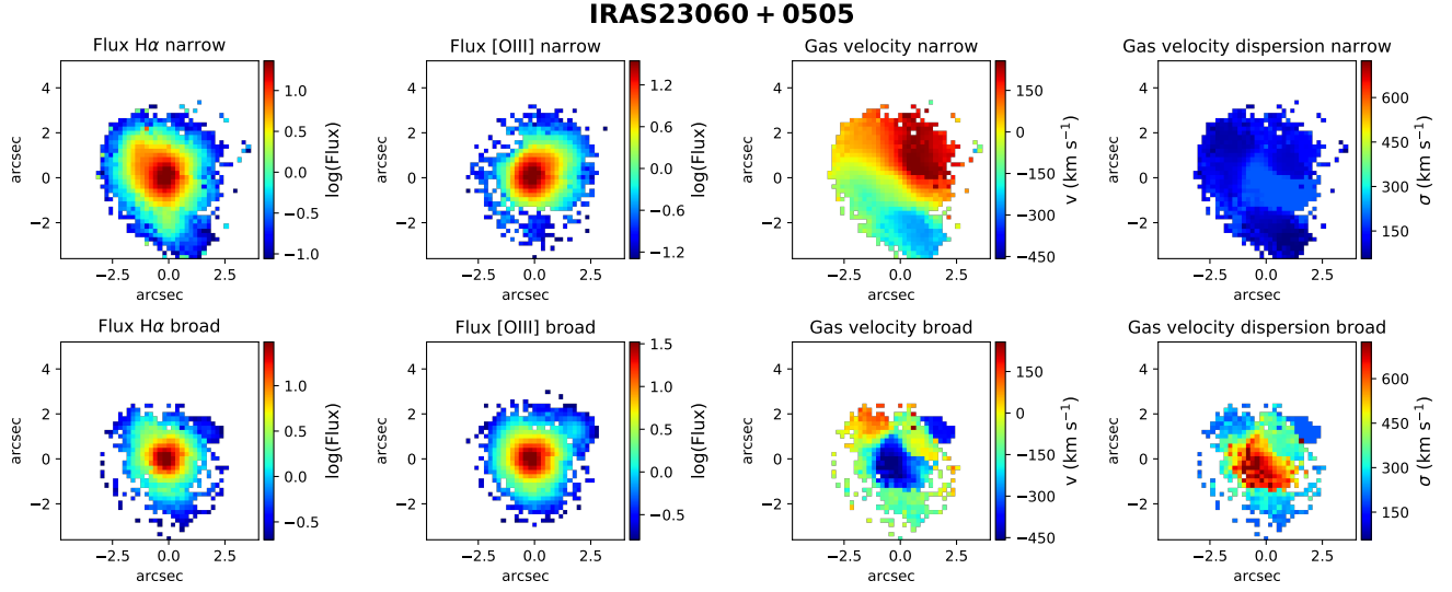
(a) Maps of the ionized gas
