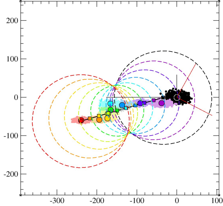
Figure 4: Validation plot for the analysis of a single transit. It is a representation of a small portion of the sky showing the different derived positions for a bright asteroid. The figure is oriented in such a way that the scan direction is vertical. The axis values are in mas. There are 10 positions, corresponding to the SM CCD (black, arbitrarily chosen as origin) and all 9 AF CCDs (rainbow colors from violet to red). The picture is supposed to show the motion in the sky of an SSO over \sim one minute (the duration of a transit). The colored circles (with solid contours) represent the measured positions converted to sky coordinates. Each of them is surrounded by a compact cloud of dots (lighter color) representing the scattering on the positions as derived from the centroiding uncertainty. The colored squares represent a fit of a linear motion to the derived positions. The dashed circles represent an error budget containing the uncertainties on the fit plus the errors on the daily attitude. Rather than showing a linear motion, the derived positions (solid circles) show a path more resembling a corkscrew motion, which deviates significantly from a linear motion, if one considers the errors on the fit of the PSF to the images alone. But if one considers also the errors on the attitude, the deviations are still well within the uncertainties. It is not clear what the origin of the corkscrew motion is, but it may imply that there is a rotational residual in the attitude with a period of the order of 1 minute and an amplitude of the order of a few tens of mas.
