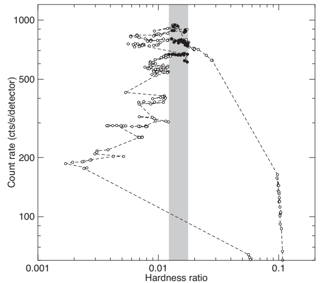
Figure 2. HID for all points shown in Fig. 1 with count rate larger than 60 cts/s/detector. The black points correspond to the data presented here, where a type-B QPO is present. The grey band shows the range in hardness spanned by the black points.
