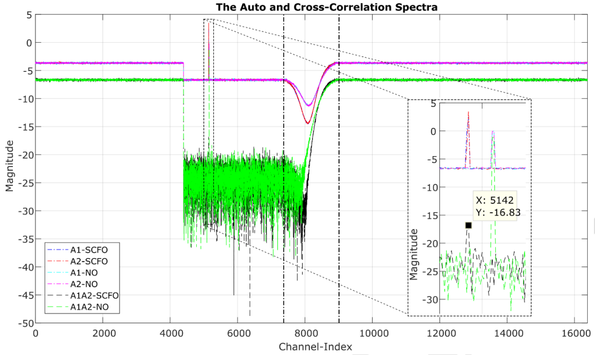
Fig. 2. Auto- and cross- correlation of imaging channels in the 5 th FS integrated for \sim 0.14 s with and without SCFO sampling for the shortest possible baseline.
