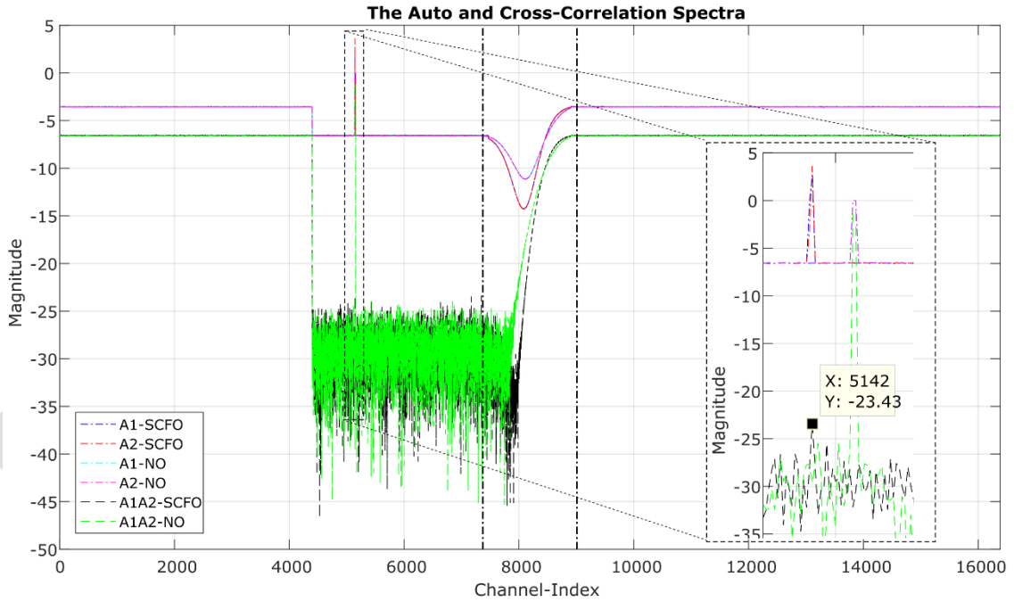
Fig. 3. Auto- and cross- correlation of imaging channels in the 5 th FS integrated for \sim 1.4 s with and without SCFO sampling for the shortest possible baseline.
