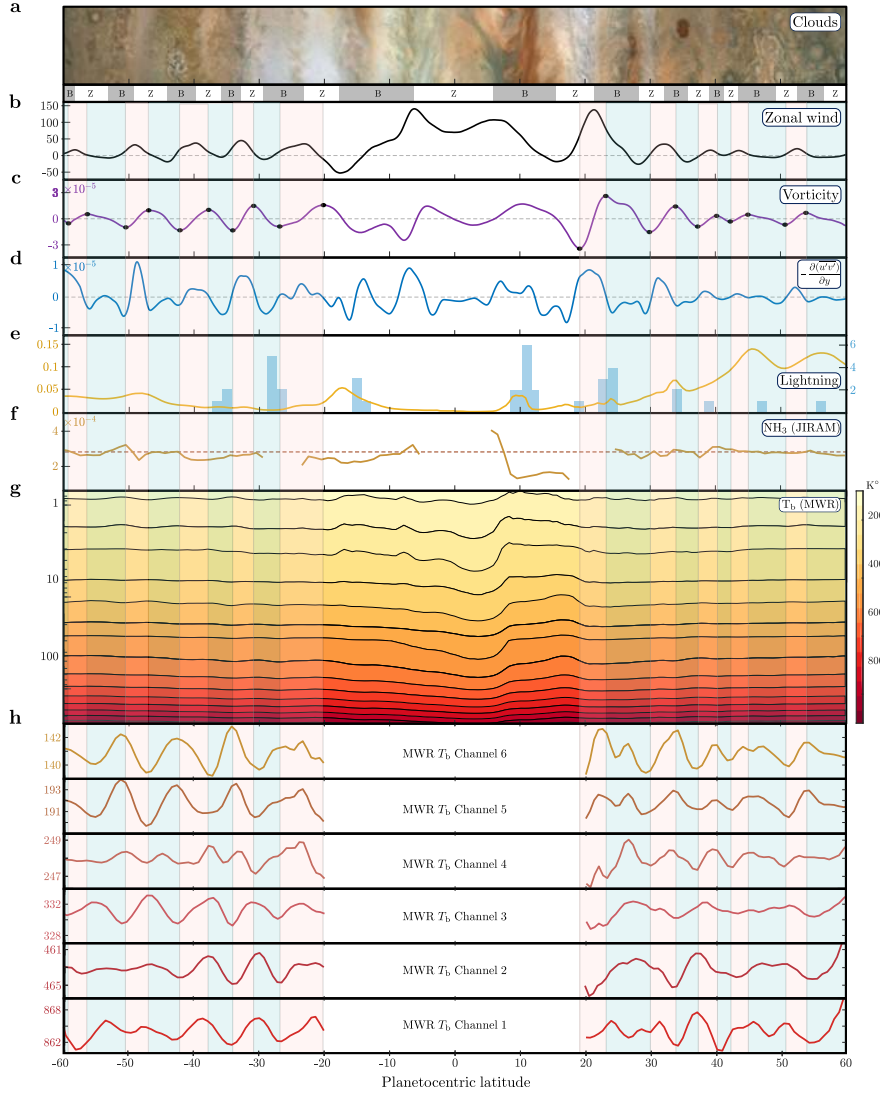
Figure 1: Observations of Jupiter’s atmosphere. (a) Image of Jupiter’s clouds (longitudes 69^{\circ} - 87^{\circ} ) taken by JunoCam on Dec. 26th 2019 during perijove 24 (image credit: NASA/JPL/SwRI/MSSS/Gerald Eichstaedt/John Rogers), with the traditional “dark” belts (“bright” zones) defined as regions of cyclonic (anticyclonic) vorticity, identified below as ‘B’ (‘Z’). (b) Jupiter’s zonally averaged zonal wind [ \pm 15 \text{ m s}^{-1} ] measured by the Hubble space telescope on December 11, 2016, during Juno’s third perijove (Tollefson et al., 2017). (c) The zonally averaged vorticity [ \text{s}^{-1} ], calculated from the zonal wind profile (panel b). Black dots represent local extrema in the midlatitudes. (d) Eddy momentum flux convergence [ \pm 2 \times 10^{-6} \text{ m s}^{-2} ] calculated from 58 image pairs taken by Cassini during its Jupiter flyby in December, 2000 (Salyk et al., 2006). (e) Lightning detections [ \text{s}^{-1} ] by Juno’s MWR during perijoves 1-8 (yellow, left axis, Brown et al., 2018) and number of lightning storms detected by the Cassini during its flyby (blue, right axis, Porco et al., 2003). (f) Distribution of ammonia [volume mixing ratio] and its mean (dashed) at a depth of \sim 6 bar, measured by Juno’s JIRAM during perijoves 1-15 (Grassi et al., 2020). (g) Nadir T_b [ ^{\circ}\text{K} ] (color) interpolated between pressure levels of 0.7 and 240 bar (vertical axis), measured by Juno’s MWR during perijoves 1-12 (Oyafuso et al., 2020). (h) Reconstructed MWR Brightness temperature at midlatitudes. A frequency filter is applied according to Eq. S7. The standard deviation of each channel and latitude is available in Fig. S3 and Fig. S4. It can be seen that T_b changes its trend at the borders between cells, consistent with the Ferrel-like cells hypothesis. (b-h) Light red (blue) bands in the midlatitudes indicate regions of positive (negative) vorticity gradients.
