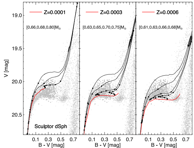
Figure 2. Optical (B-V, V) CMDs of Sculptor, zoom-in on HB stars. The grey circles display the RRL variable stars of the full sample (same as top-left panel in Fig. 1). The red lines show the zero age horizontal branch (ZAHB) from the BaSTI library (Pietrinferni et al. 2004) for different metallicities: Z = 0.0001 (left), Z = 0.0003 (middle), and Z = 0.0006 (right). The black lines display the corresponding evolutionary HB models with the labelled masses, where the overplotted circles indicate time intervals of 10 Myr. The stellar mass, at the typical colours of the RR Lyrae stars, steadily increases when moving from the brightest to the faintest HB models.
