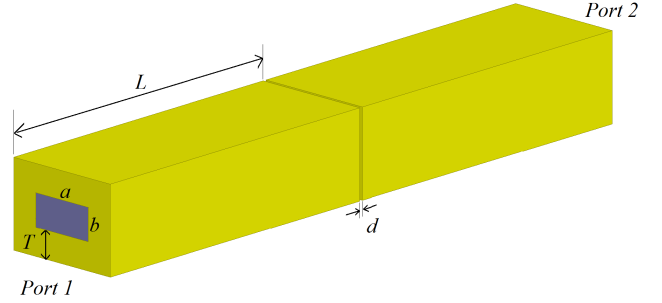
Fig. 2. Gap in a WR22 waveguide.
