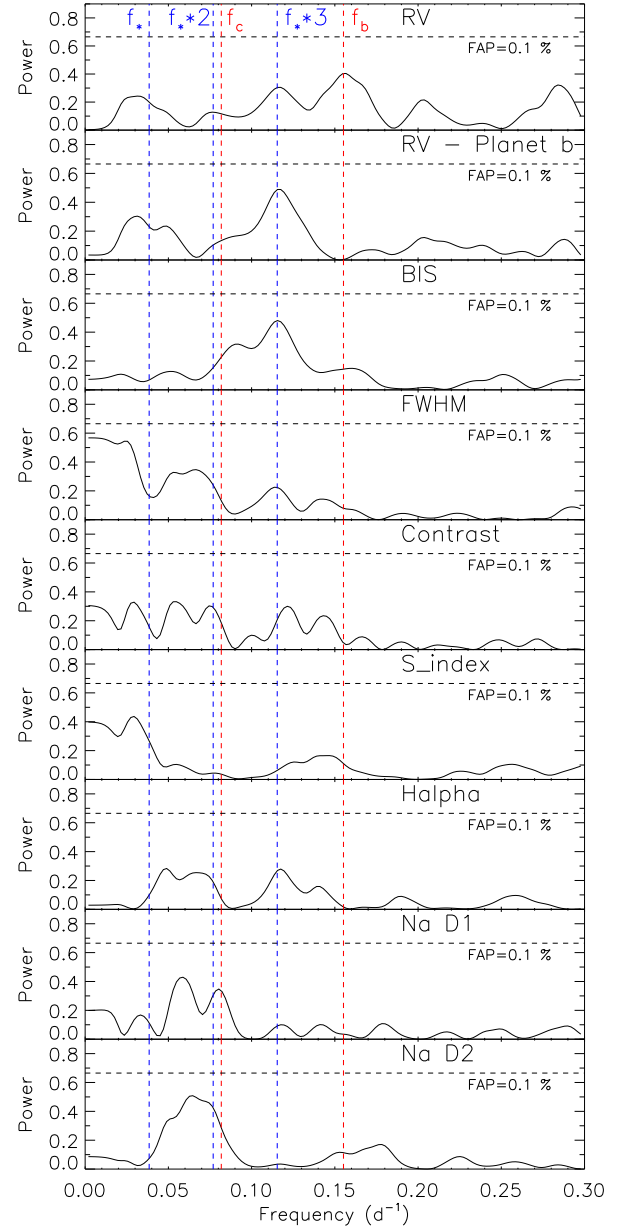
Figure C1. Generalized Lomb–Scargle periodograms of the HARPS RVs and spectral activity indicators from the HARPS DRS and TERRA. The horizontal dashed line marks the 0.1 per cent FAP level. The vertical dashed red lines mark the orbital frequencies of the two transiting planets ( f_b = 0.155 \text{ d}^{-1} and f_c = 0.082 \text{ d}^{-1} ). The vertical dashed blue lines mark the frequencies of the stellar signal at \sim 0.038 \text{ d}^{-1} and its first and second harmonics. Upper panel: HARPS DRS RVs. Second panel: RV residuals following the subtraction of the signal of TOI-1064 b. Remaining panels: the activity indicators of TOI-1064: the BIS, the FWHM, and the contrast of the CCF, the Ca II H&K lines activity indicator (S-index), H \alpha , Na D1, and Na D2.
