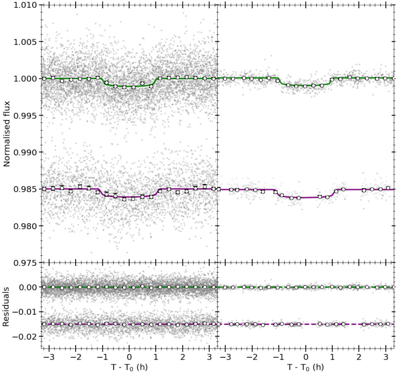
Figure 8. Top panels: detrended TESS (left) and CHEOPS (right) photometry phase-folded to the orbital periods of planets b and c (offset by -0.015 for clarity). Unbinned data are shown in grey, with fluxes binned every 15 min given as white circles. The best-fitting transit models for TOI-1064 b and TOI-1064 c are presented in green and purple, respectively. Bottom panels: residuals to the fits shown in the top panels with the same colouration.
