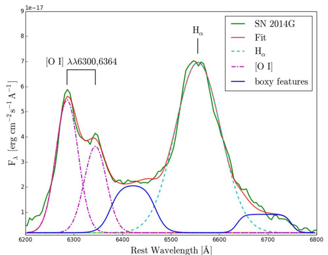
Figure 11. Modelling of the 6200–6800 Å region of the SN 2014G spectrum at 342 d. We used Gaussian profiles to reproduce H\alpha and the [O I] \lambda\lambda 6300, 6364 doublet and a boxy profile to reproduce the ‘bridge’ in between.
