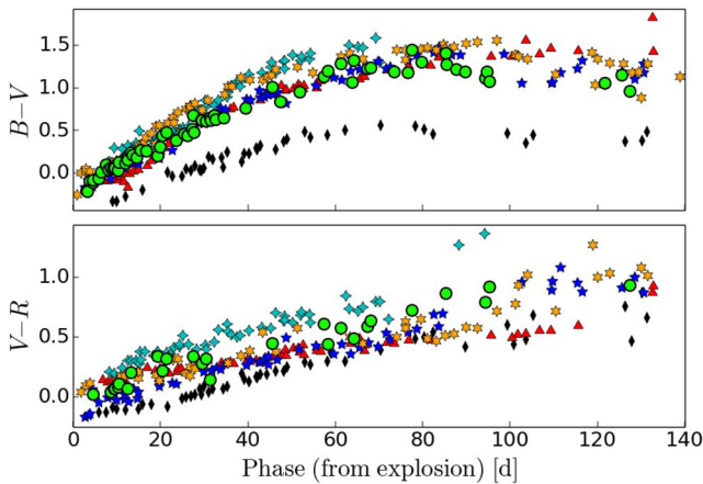
Figure 4. B - V and V - R extinction-corrected colour evolution of SN 2014G compared to the other SNe considered in the text. The legend is the same as in Fig. 3.
