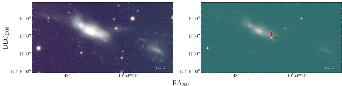
Figure 1. RGB images of the SN 2014G field. On the left, a reference image where the whole system Arp 205 (NGC 3448+UGC 6016) is clearly visible. On the right, a post-explosion image, where SN 2014G is marked in red.
