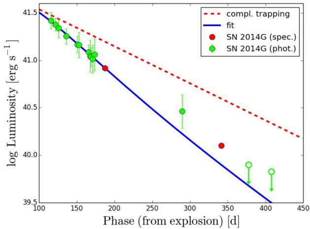
Figure 12. Zoom in of the radioactive tail of SN 2014G. The green points correspond to the uvoir bolometric LC, while the red ones are the integrated flux from the spectra. The red dashed line represents where the LC would be if it followed the ^{56}\text{Co} decay in a full trapping regime. The blue solid line is the fit to the data with equation (2). The luminosities extrapolated from the spectra have high uncertainties, thus were not included in the fit.
