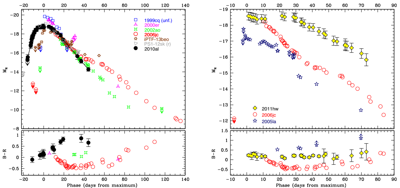
Figure 4. Top-left: R -band absolute light curves of SN 2010al and other Type Ib/Ic SNe, including SNe 1999cq, 2000er, 2002ao, 2006jc, PS1-12sk and iPTF-13beo (Matheson et al. 2000; Foley et al. 2007; Pastorello et al. 2007, 2008a; Sanders et al. 2013; Gorbikov et al. 2014). SN 2010al is marginally fainter at peak than other SNe Ib/Ic shown here, and has a slower rise to maximum. Bottom-left: B − R colour curves for the same sample of SNe Ib/Ic. Top-right: R -band absolute light curves of the Type Ib/Ic SNe 2011hw and 2005la, compared with the prototypical SN Ib/Ic 2006jc. For SNe 2011hw and 2005la, we adopt the discovery epochs as reference dates for the maximum. For SN 2005la, only the most significant detection limits are shown. Bottom-right: B − R colour curves for SNe 2011hw, 2005la and 2006jc. Data have been corrected for interstellar reddening.
