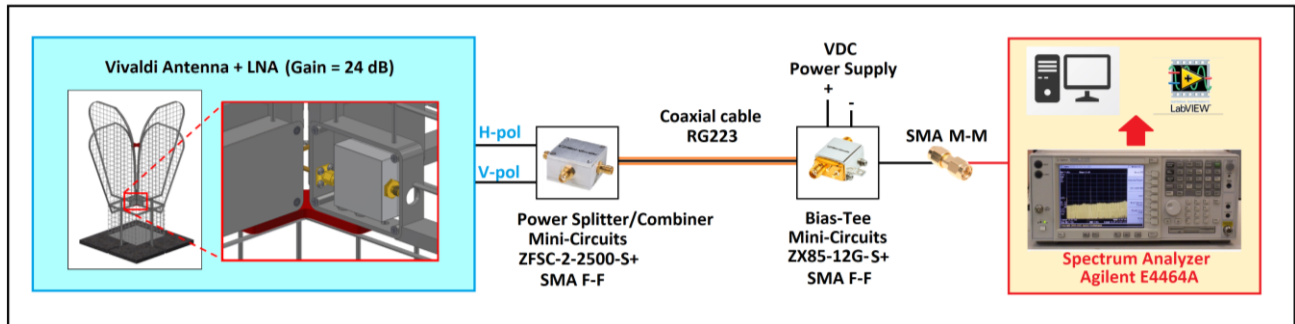
Figure 3. Schematic of the RFI monitoring system.
