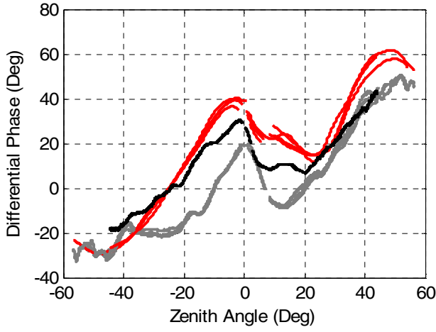
Fig. 4. Differential phase patterns between element 2 and element 42 at 57 MHz. Measurement in quasi far-field condition (black curve) and near-field measurements (grey curves) are compared with simulations (red curves).
