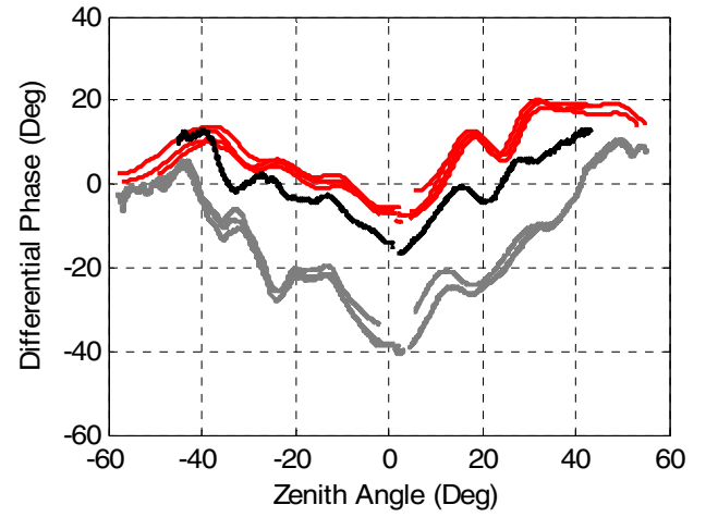
Fig. 5. Differential phase patterns between element 26 and element 42 at 57 MHz. Measurement in quasi far-field condition (black curve) and near-field measurements (grey curves) are compared with simulations (red curves).
