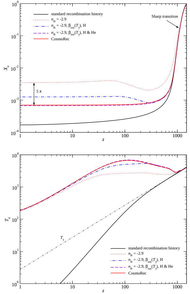
Figure 1. Effect of heating by decaying magnetic turbulence on the ionization history (upper panel) and electron temperature (lower panel) for B_0 = 3 \text{ nG} and n_B = -2.9 .
