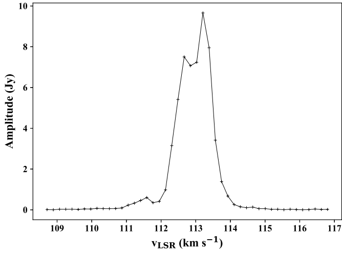
(i) 6.7 GHz methanol maser – G030.70–00.06 (second epoch)
