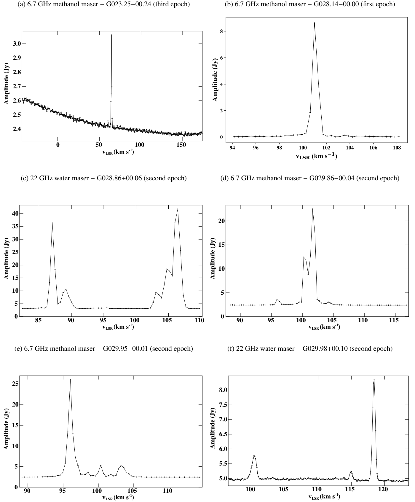
Fig. B.1: Spectra of the 16 maser sources listed in Table 1. Each spectrum is an amplitude scalar average of one-second integrations of all data on all baselines.
