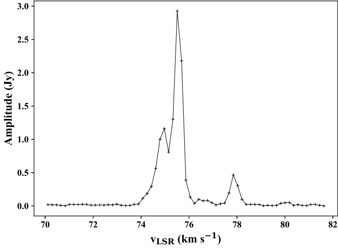
(o) 6.7 GHz methanol maser – G032.04+00.05 (second epoch)
