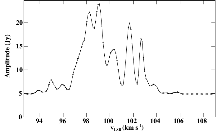
(p) 6.7 GHz methanol maser – G033.09–00.07 (second epoch)
