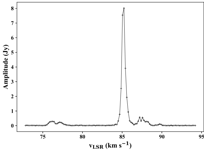
(k) 6.7 GHz methanol maser – G030.78+00.20 (second epoch)
