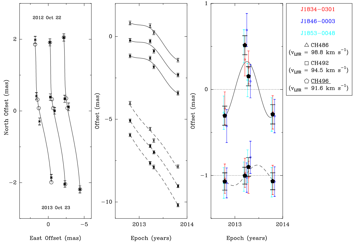
(h) 6.7 GHz methanol maser – G030.74–00.04
