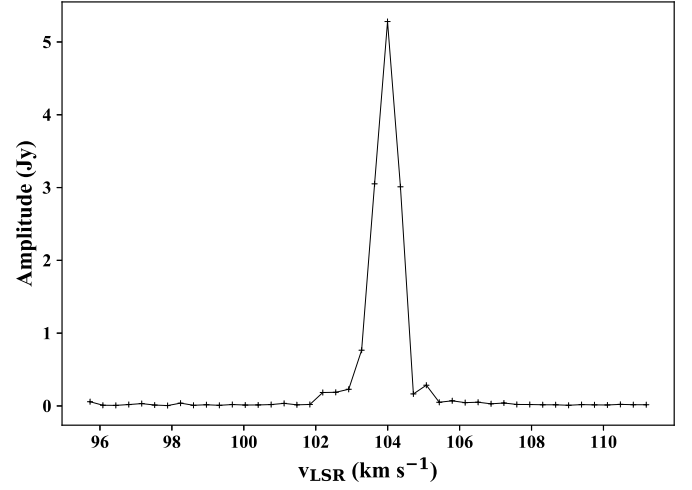
(p) 6.7 GHz methanol maser – G033.09–00.07 (second epoch)
