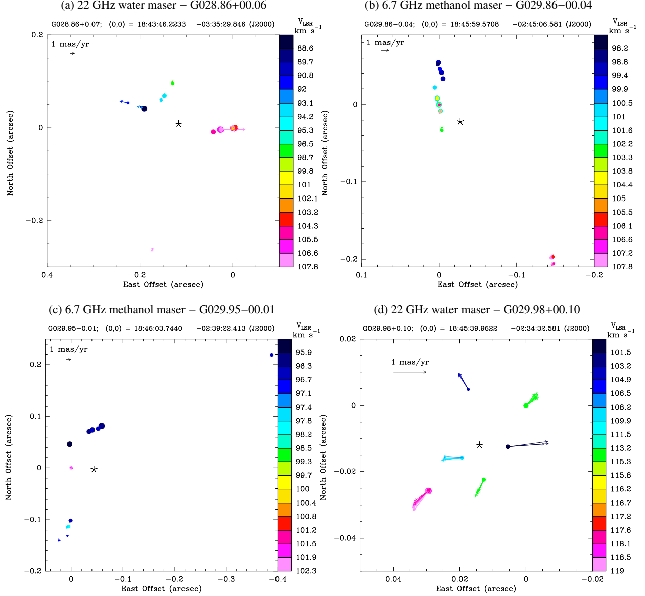
Fig. D.1: Internal motion plot. The star symbol indicates the position of the central object.
