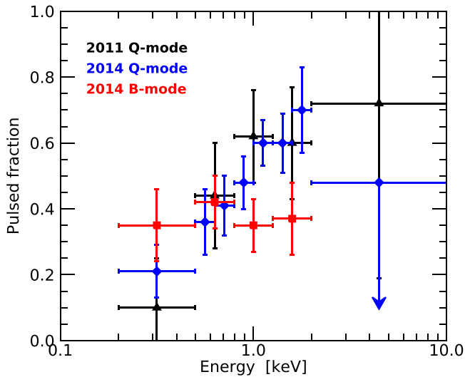
Figure 1. Pulsed fraction of PSR B0943+10 as a function of energy, as measured by Hermesen et al. (2013; Q-mode: black triangles) and by Mereghetti et al. (2016; Q-mode: blue diamonds, B-mode: red squares).
