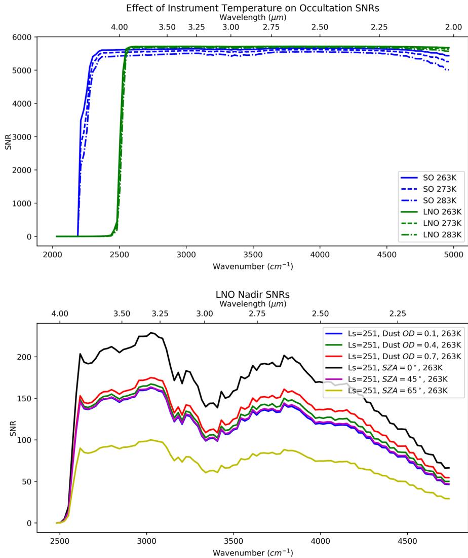
Fig. 6 Overview of the expected SNR for the SO and LNO spectrometers in solar occultation and nadir mode respectively, from Thomas et al. (2016). Top: the SNR in solar occultation mode assumes no dust extinction and an optimal integration time matched to the instrument sensitivity; values are given for three different temperatures of the instrument (263 K, 273 K, 283 K). Bottom: SNR of nadir observations by LNO for a range of observation conditions: dust optical depth = 0.1, 0.4, and 0.7 or solar zenith angles of 0, 45, and 65°; L_S = 251^\circ [close to Sun], assuming a planetary albedo of 0.242 and all 144 detector pixels are binned for a Mars observation of 15 seconds duration
