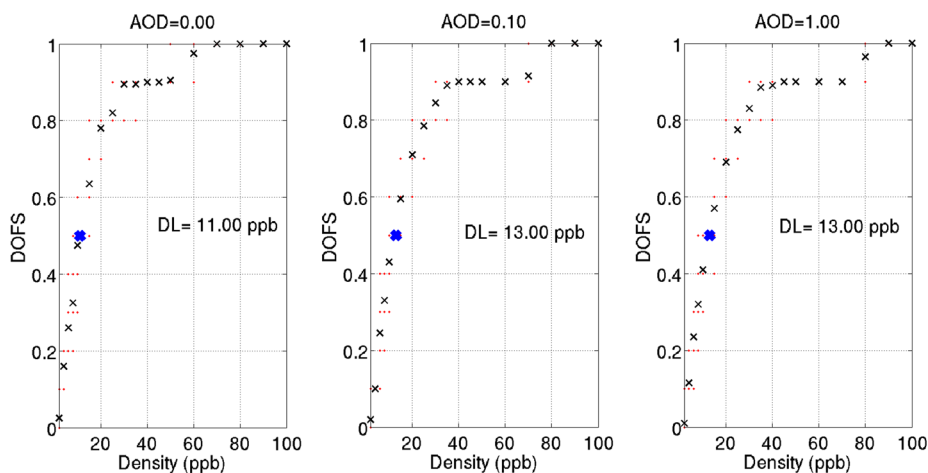
Fig. 28 Detection Limits for \text{CH}_4 in three scenarios of dust: \text{AOD} = 0 (left), \text{AOD} = 0.1 (center) and \text{AOD} = 1.0 (right). These results were obtained by retrieving methane in the diffraction order 134 i.e. spectral interval from 3011 to 3036 \text{ cm}^{-1} . The red dots show the 20 individual results. The 18 black markers indicate the mean Degree of Freedom of the Signal (DOFS) per factor tested. The DOFS equals to 0.5 is represented by the blue marker
