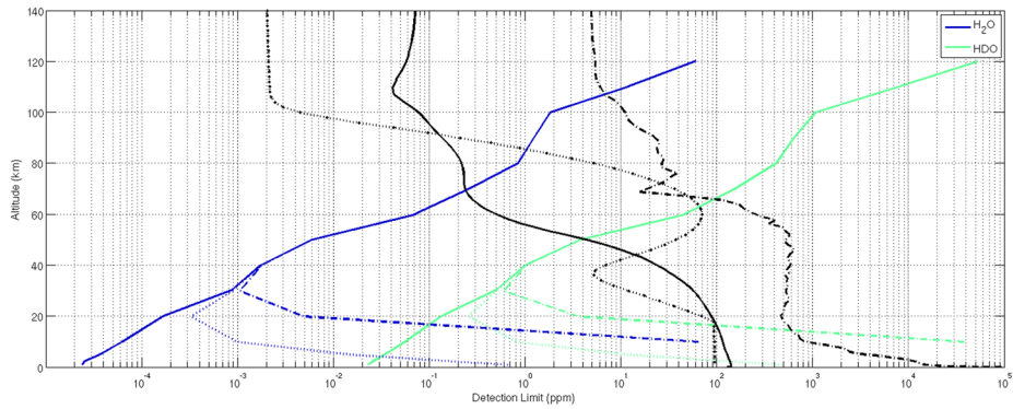
Fig. 21 Detection limits of \text{H}_2\text{O} and its isotopologue HDO, considering an enrichment of 5.6 of HDO compared to the SMOW value on Earth. The detection limits are given for several dust loadings, here expressed as Aerosol Optical Depth (AOD): solid: AOD = 0.0, dotted: AOD = 0.1, and dash-dotted: AOD = 1.0. The black lines represent results from different models: solid is the yearly average obtained by GEM-Mars; dash-dotted: profile made up of the maximum value calculated by the model at each altitude; dotted: profile used in Chaffin et al. (2017) as being representative of the high-altitude water profiles observed by SPICAM (Maltagliati et al. 2011)
