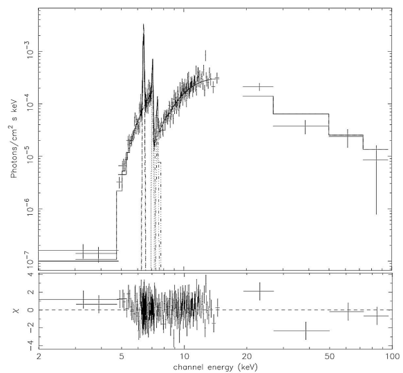
Figure 10: XMM-Newton and ISGR1 unfolded photon spectra of IGR J16318–4848, the first new source detected by INTEGRAL and an extremely absorbed HMXB. From Walter et al. (2003).
