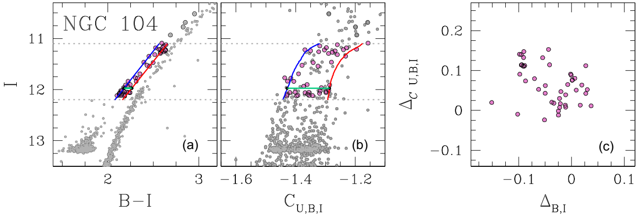
Figure 15. This figure illustrates the procedure to derive the ChM of AGB stars in NGC 104 (47 Tucanae). Panels (a) and (b) represent the I versus B-I and I versus C_{U,B,I} diagrams, respectively. The red and blue lines mark the boundaries of the AGB sequence, while the aqua segments indicate the width of the AGB sequence. AGB stars are marked with dots. Only AGB stars between the two horizontal (pink dots) lines are used to derive the ChM plotted in panel (c).
