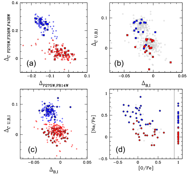
Figure 10. Upper panels: \Delta_{C F275W, F336W, F438W} versus \Delta_{F275W, F814W} ChM of NGC 288 from HST photometry (Milone et al. 2017a). The probable 1G and 2G stars selected by Milone and collaborators are coloured red and blue, respectively (upper left-hand panel). Reproduction of the \Delta_{C U,B,I} and \Delta_{B,I} ChM derived in Fig. 7. Large squares represent stars with both HST and ground-based photometry (upper-right). Bottom panels: The 1G and 2G stars identified in the \Delta_{C U,B,I} and \Delta_{B,I} plane are represented with red and blue circles, respectively, in the bottom left-hand panel ChM. Sodium versus oxygen abundances for RGB stars of NGC 288 (Carretta et al. 2009). Stars for which [O/Fe] estimates are not available are plotted on the right-hand side of the vertical line in the panel. Stars included in the ChM for which sodium abundances are available are represented with large dots.
