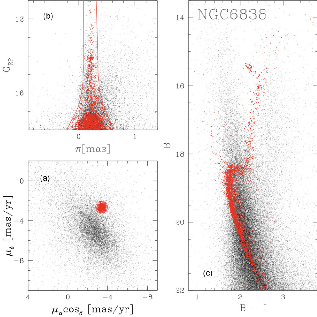
Figure 1. This figure illustrates the procedure to select probable members of NGC 6838. Panel (a) shows the VPD of proper motions for stars in the cluster field. Panel (b) show G_{RP} as a function of the parallax \pi and the two lines drawn by eye that encloses probable cluster members. The B versus B - I CMD is illustrated in panel (c). Cluster members selected are represented with red symbols.
