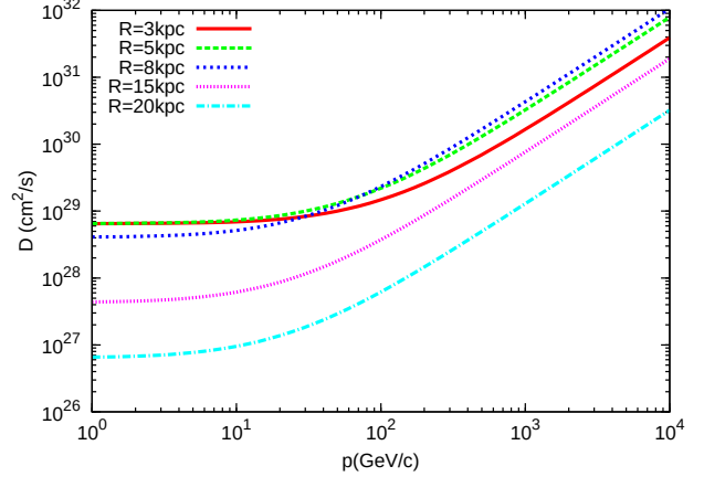
Figure 3. Diffusion coefficient D(z=0, p) as a function of momentum in GeV/c for different Galactocentric distances as labelled.
