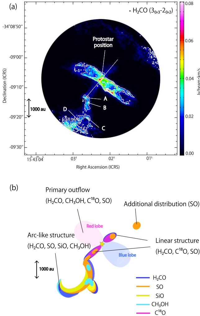
Figure 1. (a) Moment 0 map of the H 2 CO line emission. Contour levels are every \sigma from 3\sigma , where \sigma is 6 mJy beam -1 . The line intensities are integrated from 3.7 to 5.7 km s -1 to focus on the arc-like feature and linear structure. White cross marks show the five locations where molecular line profiles are produced (see Figure 3). The circle at top right represents the synthesized beam size. The dashed arrow represents the direction of the PV diagram. (b) Schematic picture of the molecular distributions.
