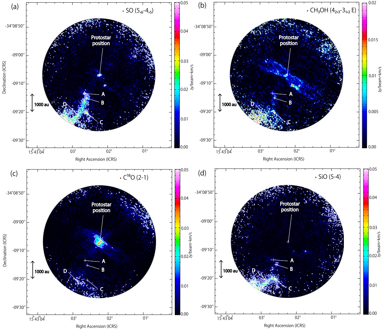
Figure 2. (a)–(d) Moment 0 maps of the SO, CH 3 OH, C 18 O, and SiO line emission. Contour levels are every \sigma from 3\sigma , where \sigma is 4 mJy beam −1 km s −1 , 3 mJy beam −1 km s −1 , 4 mJy beam −1 km s −1 , and 3 mJy beam −1 km s −1 , respectively. See Figure 1 caption for additional details.
