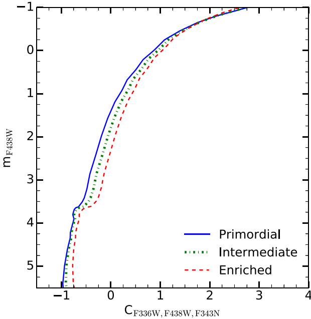
Figure 2. Isochrones of a 10 Gyr old stellar population in the m_{F438W} versus C_{F336W, F438W, F343N} CMD, showing the upper part of the MS as well as the RGB. The blue solid line corresponds to a population with primordial composition, whereas the green dash-dotted line shows stars with an intermediate enriched composition and the red dashed line shows enriched stars (see the text for more details).
