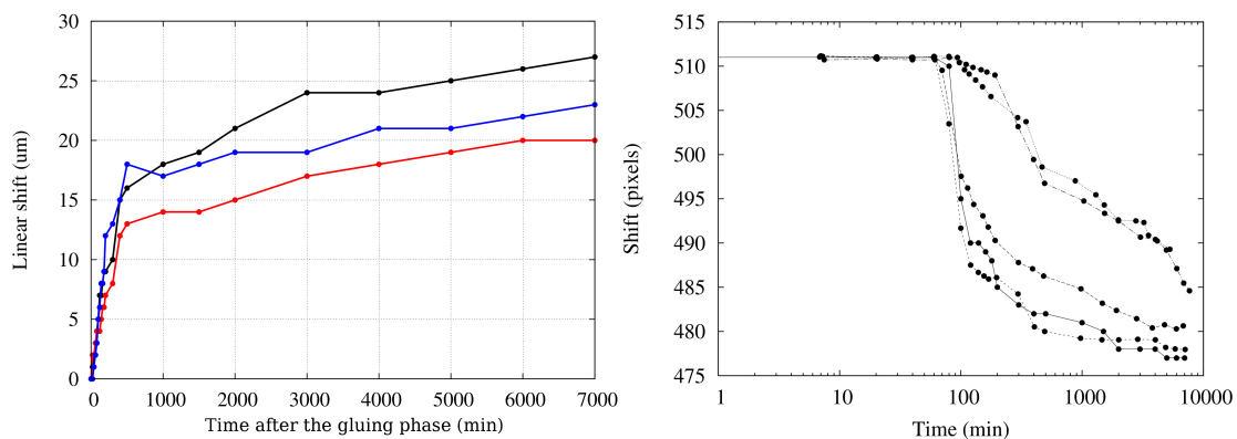
Figure 4. left : The linear shift of a crystal measured with the optical camera, as a function of time. The total shift (20–25 \mu\text{m} ) corresponds to a combination of rotation and translation of the crystal by the glue shrinkage. right : Shift of the diffracted image (in detector pixels) measured with the X-ray beam as a function of time for 5 different crystals glued over a carbon fiber support. The glue injection was made through a hole performed through the support.
