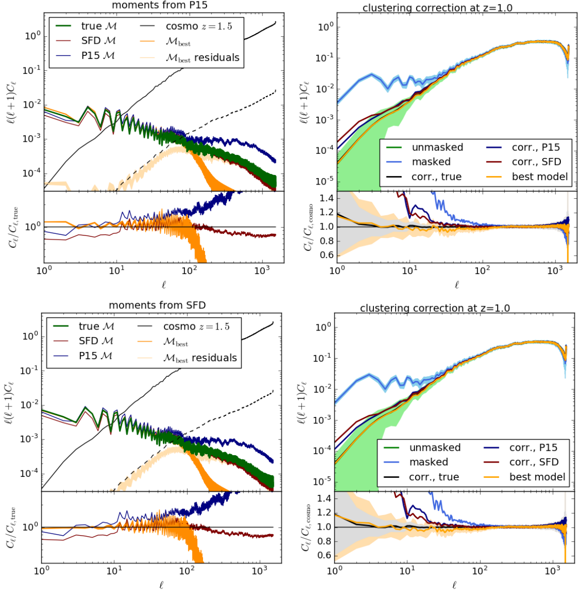
Figure 12. Angular clustering of best reconstruction for the mask (left panels) and reconstructed angular clustering of galaxies (right panels) for reconstructions that use \langle \mathcal{M} \rangle and \langle \mathcal{M}^2 \rangle from P15 (upper panels) and SFD (lower panels). Symbols and colors are as in figures 6 and 8.
