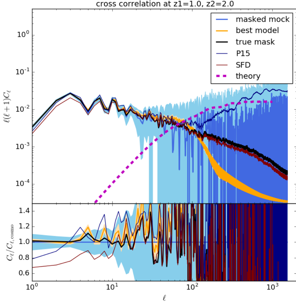
Figure 10. Angular cross-correlation of masked catalog for z_1 = 1.0 and z_2 = 2.0 . The green and blue line gives the average measurement of the masked catalog, lighter blue areas gives its sample variance (16th and 84th percentiles). Orange, black, dark blue and maroon lines give the average of the predicted cross-correlation using respectively the best reconstruction, the true P13 mask, the P15 and SFD masks. The lower panels give the residual with respect to the average true cross correlation.
