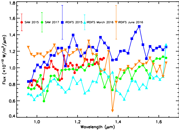
Fig. 2. Comparison among the extracted spectra for HD142527B obtained by both direct imaging and SAM modes of SPHERE in the IFS wavelength range ( 0.95 - 1.65 \mu\text{m} ). In the upper part of the plot is indicated the value of the average value of the error for each spectrum. The SAM IFS spectrum taken in 2015 is limited to the YJ band of IFS ( 0.95 - 1.35 \mu\text{m} ). For a clearer view of the plot all points are connected by continuous lines.
