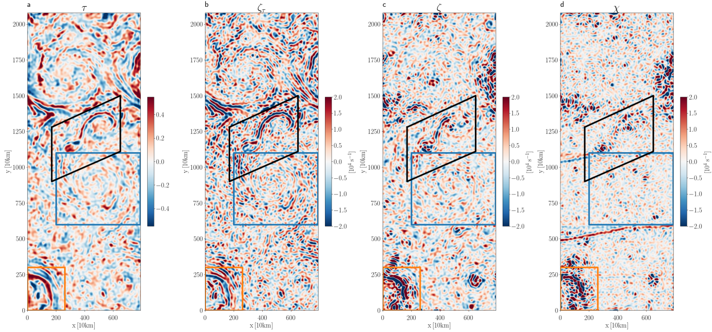
Extended Data Figure 4. Band pass filtered \tau , \zeta\tau , \zeta and \chi between 250 and 1,600 km Maps of filtered a) \tau , b) \zeta\tau , c) \zeta and d) \chi after application of a band pass filter that retains lengthscales between 250 and 1,600 km (see Methods). The region delineated by the black polygon comprises the streamer subdomain joining two intermediate-scale anticyclones that is discussed in the main text. The blue rectangle comprises the polar vortex and the orange rectangle captures filamentary structures surrounding one of the circumpolar cyclone. These subdomains are analyzed in Extended Data Figs. 5–7.
