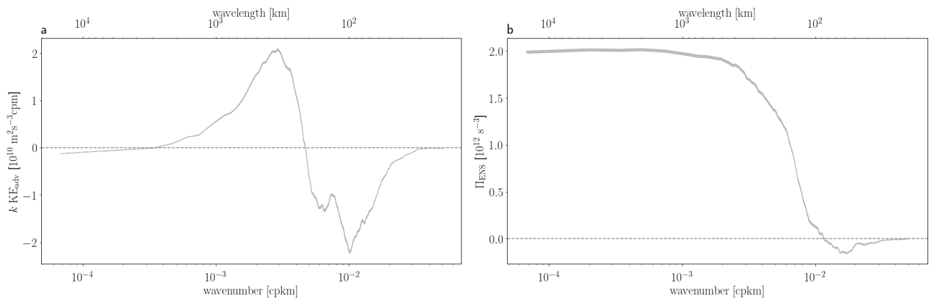
Extended Data Figure 13. Error envelope for a) KE and b) enstrophy transfers using wind field n0103. Same methodology as Extended Data Figure 12 but applied to Figure 4. The error associated with the wind measurements does not impact the transfers computation.
