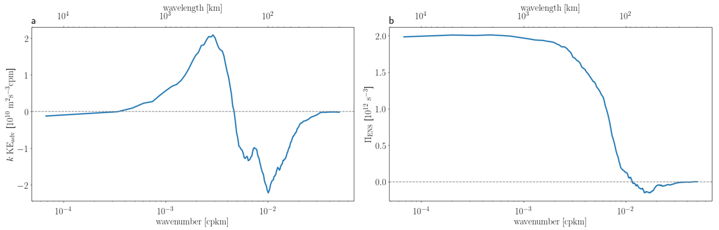
Figure 4. Spectral fluxes derived from the wind measurements a) KE transfer in variance preserving form ( k \text{KE}_{\text{adv}} ). Positive (negative) k \text{KE}_{\text{adv}} indicates an energy gain (loss). Scales smaller (larger) than 215 km lose (gain) energy, corresponding to an upscale energy transfer. b) Enstrophy spectral flux (see Methods) showing an ubiquitous direct cascade from large to small scales, consistent with an upscale KE transfer in classical theory of rotating turbulence 37 .
