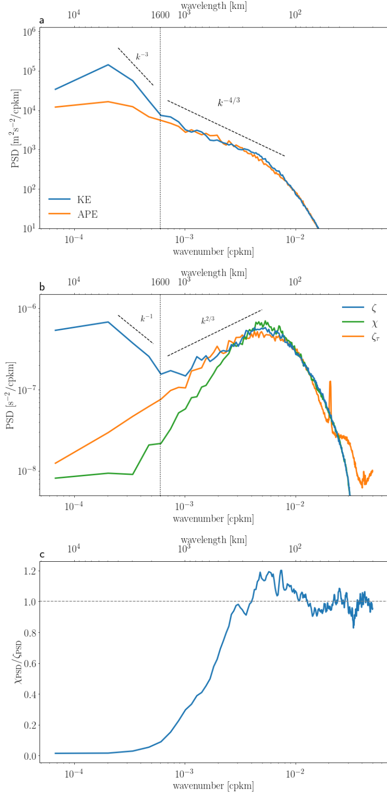
Figure 3. Spectral characteristics a) Spectra kinetic energy (KE, blue curve) and available potential energy (APE, orange curve). b) Power spectra of relative vorticity ( \zeta , blue curve), horizontal divergence ( \chi , green curve) and vorticity derived from \tau ( \zeta_\tau , orange curve). See Extended Data Fig. 2 for \zeta and \chi in physical space. A spectral slope discontinuity in KE and \zeta occurs at 6 \cdot 10^{-4} cpkm ( \sim 1,600 km), highlighted by the vertical dashed line. Thick dashed lines show spectral slopes. c) \chi to \zeta power spectra ratio \chi_{\text{PSD}} / \zeta_{\text{PSD}} .
