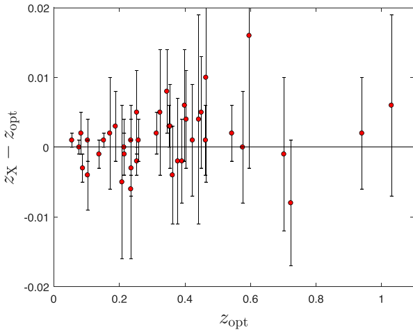
Figure 3. The difference between X-ray redshift and optical redshift of all clusters.
