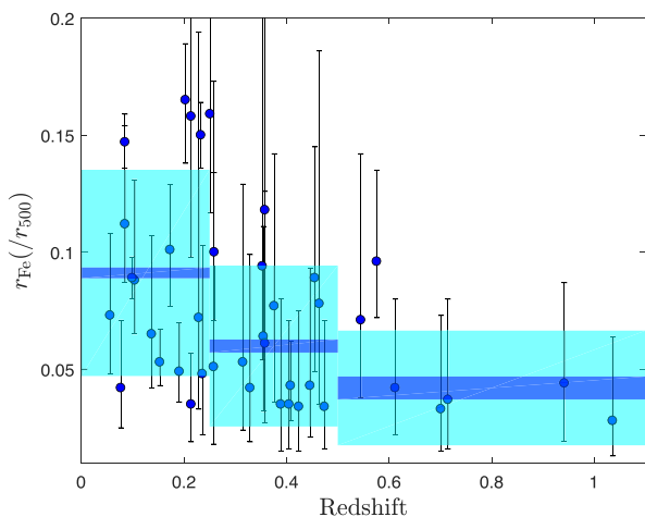
Figure 8. The scale of the iron excess peak, r_{\text{Fe}} , plotted versus redshift. The blue and cyan shaded areas show the weighted average and r_{\text{ms}} in three redshift bins, respectively.
