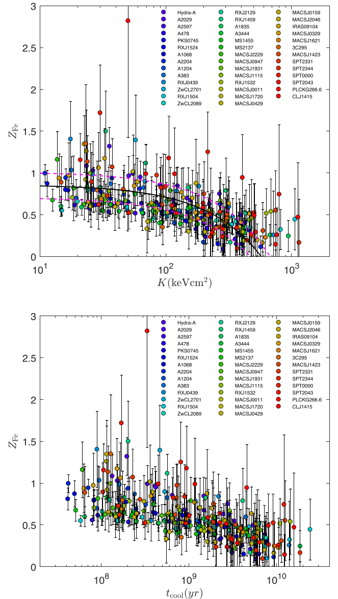
Figure 5. Upper panel: The distribution of Z_{\text{Fe}} versus K(kT, n_e) of all the measured bins in the clusters. The colour code denotes the redshift of the clusters, from the lowest (blue) to the highest (red). The solid line is the best-fitting linear model. The dashed lines show the rms dispersion of the distribution. Lower panel: The distribution of Z_{\text{Fe}} versus the cooling time t_{\text{cool}} .
