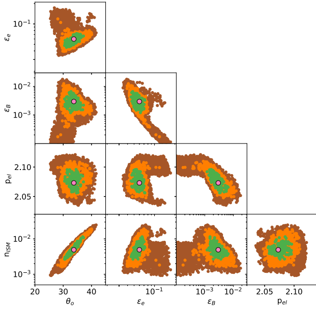
FIG. 4. Corner plot showing the degeneracy of the fit parameters for the structured jet model. A strong degeneracy is evident between the interstellar density and the observing angle. The meaning of different colors is the same as in Fig. 3.
