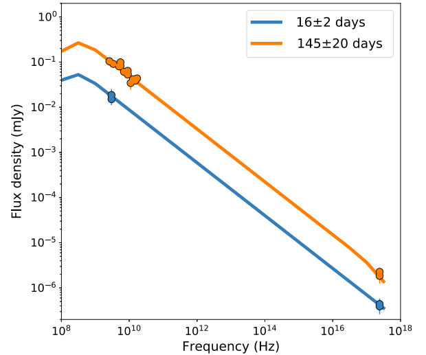
FIG. 7. Broadband spectra of the transient produced by the external shock from a structured jet seen off axis. The afterglow spectrum from the radio to the x rays is shown at two epochs. In blue is the time of the earliest radio and x -ray measurements ( \sim 16 days after the trigger); in orange is the epoch at which the radio light curve peaks, approximately 145 days after the trigger. The displayed data have been taken within a few days of the time at which the spectra were computed (as specified in the legend).
