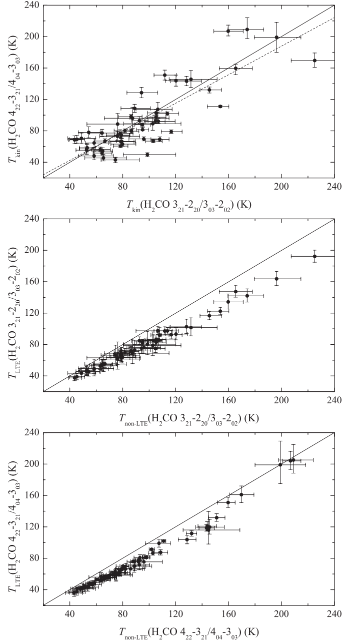
Fig. 5. Top panel: Comparison of kinetic temperatures derived from para- \text{H}_2\text{CO} 3_{21}-2_{20}/3_{03}-2_{02} and 4_{22}-3_{21}/4_{04}-3_{03} ratios. The dashed line is the result from an unweighed linear fit, T_{\text{kin}}(4_{22}-3_{21}/4_{04}-3_{03}) = (0.9 \pm 0.1) \times T_{\text{kin}}(3_{21}-2_{20}/3_{03}-2_{02}) + (5.8 \pm 7.8) , with a correlation coefficient, R , of 0.85. Middle and bottom panels: Comparisons of kinetic temperatures derived from LTE and RADEX non-LTE calculations for para- \text{H}_2\text{CO} 3_{21}-2_{20}/3_{03}-2_{02} and 4_{22}-3_{21}/4_{04}-3_{03} ratios, respectively. The temperature uncertainties are obtained from observed para- \text{H}_2\text{CO} line ratio errors. Solid lines indicate equal temperatures.
