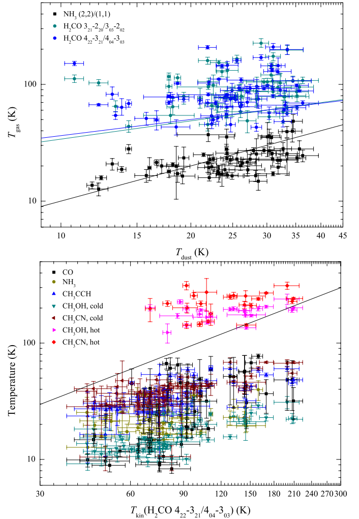
Fig. 8. Top panel: Comparison of kinetic temperatures derived from para-H 2 CO ( 3_{21}-2_{03}/3_{03}-2_{02} and 4_{22}-3_{21}/4_{04}-3_{03} , cyan and blue points) and NH 3 ( 2,2 )/(1,1) (black squares) ratios against the dust temperatures. NH 3 kinetic temperatures are selected from Wielen et al. (2012). The cyan and blue straight lines are the results from unweighed linear fits for gas temperatures derived from para-H 2 CO ( 3_{21}-2_{03}/3_{03}-2_{02} and 4_{22}-3_{21}/4_{04}-3_{03} , respectively). Bottom panel: Comparisons of gas temperatures derived from para-H 2 CO ( 4_{22}-3_{21}/4_{04}-3_{03} ), CO, NH 3 ( 2,2 )/(1,1), CH 3 OH, CH 3 CN, and CH 3 CCH. Temperatures of CO, CH 3 OH, CH 3 CN, and CH 3 CCH are taken from Giannetti et al. (2017). The black straight lines in both panels indicate equal temperatures.
