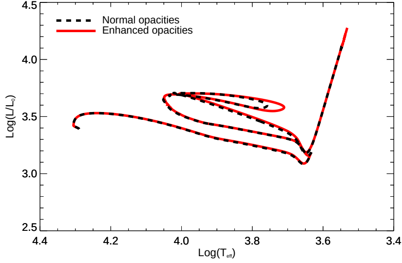
Figure 2. Evolutionary tracks for a 7M_{\odot} star with a Z = 0.008 ; Y = 0.256 composition. Solid red line: enhanced opacities. Dashed black line: normal opacities.
