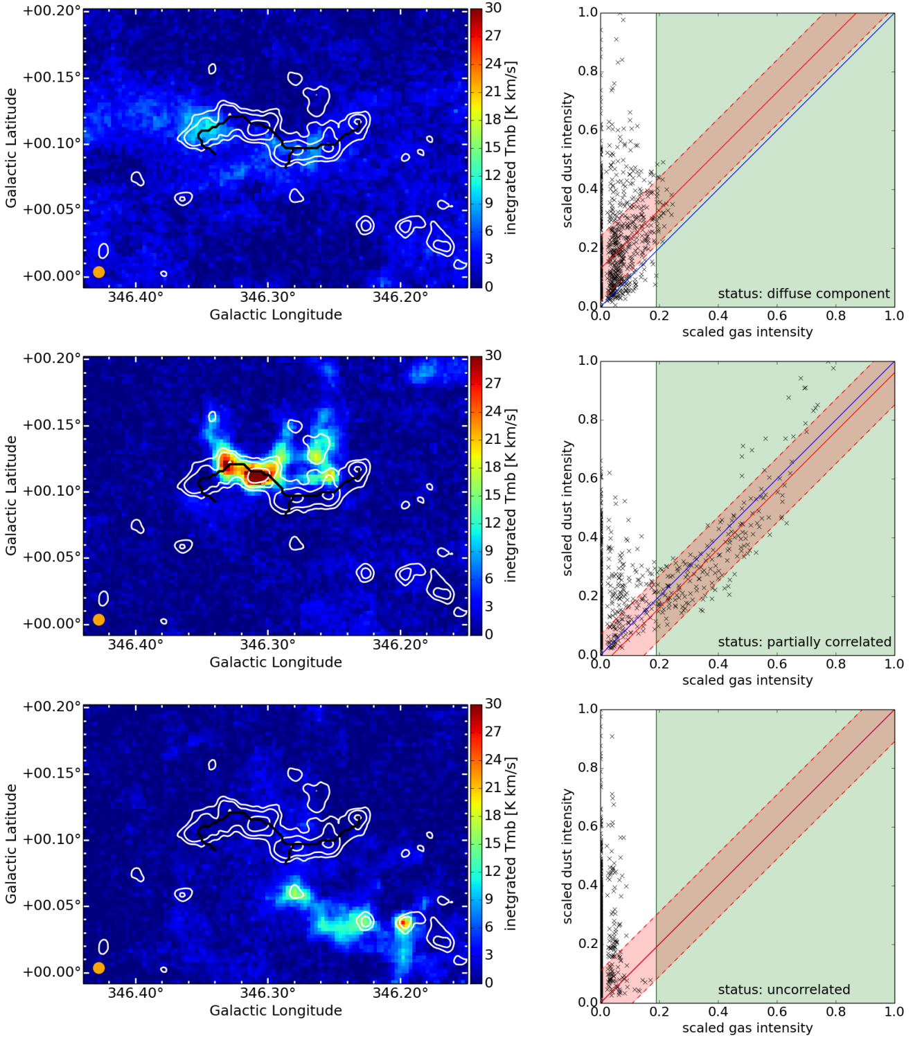
Fig. A.5. Integrated ^{13}\text{CO} intensity maps (left) and gas-dust correlation plots (right, description as in Fig. A.2)) of the second (top), third (middle), and fourth (bottom) velocity component of the filament candidate "G346.293+00.109". The second, diffuse component is listed as "G346.293+00.109_1" and the third, partially correlated component is listed as "G346.293+00.109_2". The uncorrelated component is not listed in the catalogue. The first velocity components of the candidate is shown in Fig. A.4.
