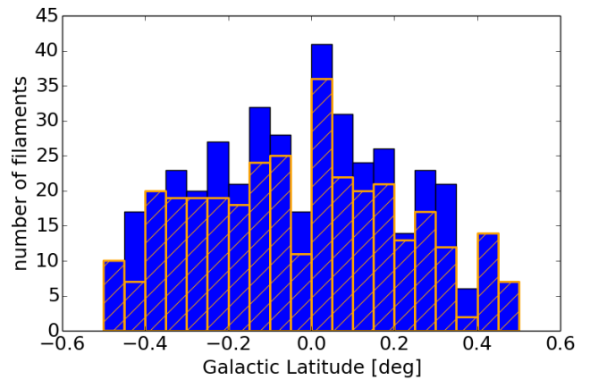
Fig. 11. Distribution of the filament positions in Galactic Latitude. The orange hatch marks the filaments with distance estimate.
