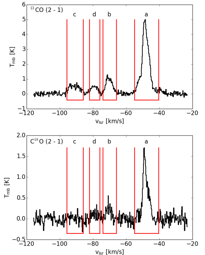
Fig. 3. Average ^{13}\text{CO} (top) and \text{C}^{18}\text{O} (bottom) spectrum over the skeleton of filament candidate G333.297+00.073 (see Figs. 1 and 2). The red lines mark the identified emission intervals named by letters.
