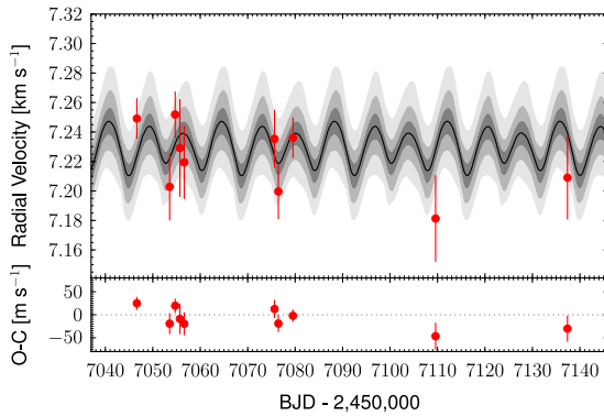
Figure 2. SOPHIE RVs as a function of time and the corresponding residuals. The overplotted black curve is the median value of the distribution of models (described in Section 4) corresponding to 1000 random MCMC steps, and the different shades of grey represent the 68.3, 95.5, and 99.7 per cent Bayesian confidence intervals.
