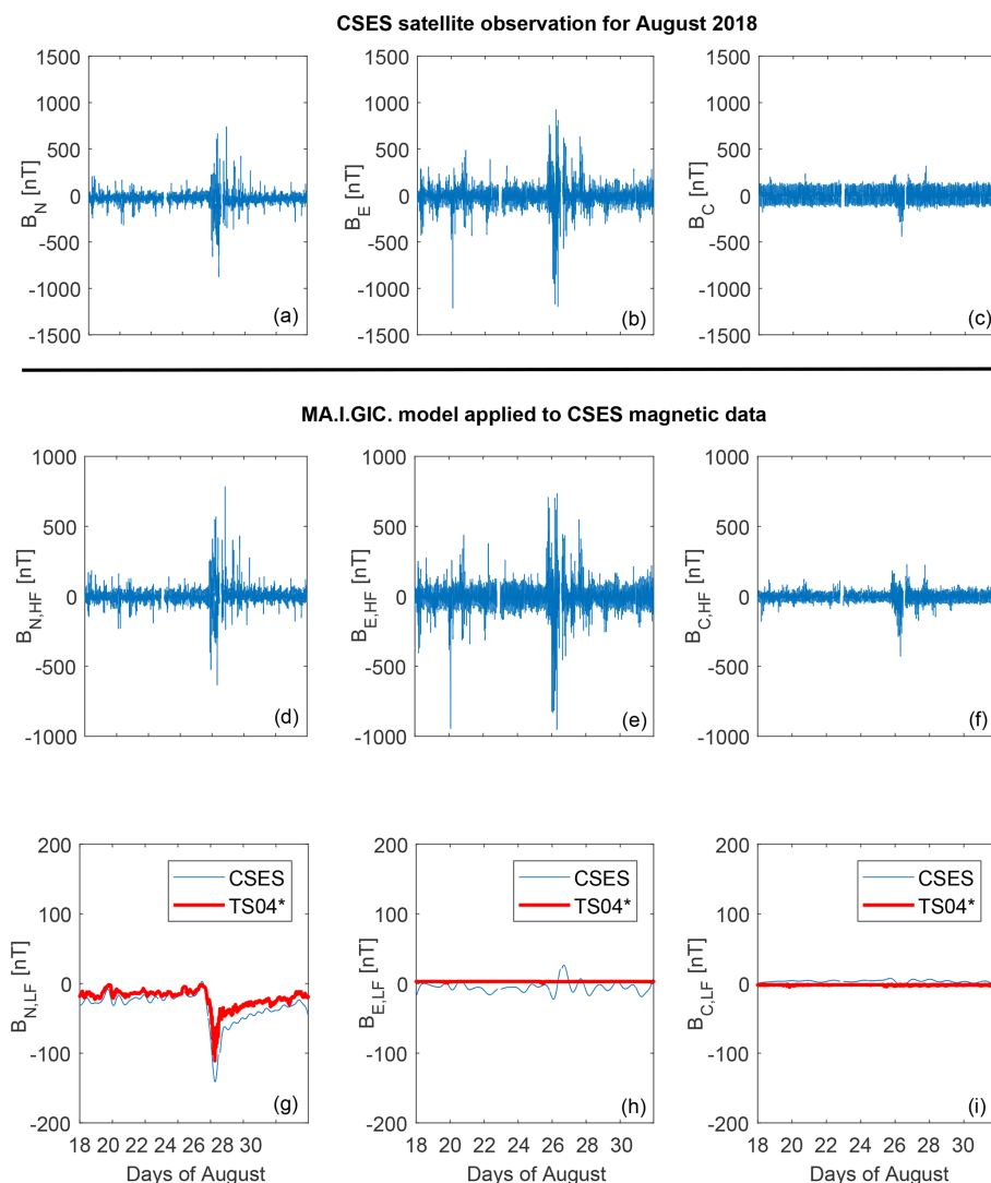
Figure 5. Magnetic field observations at the CSES orbit along geographic north–south (a), east–west (b) and vertical (c). MA.I.G.I.C. model applied to CSES magnetic data: panels (d–f) show the high-frequency timescales ( \sim 25 \mu\text{Hz} < f < 3 \text{ mHz} ; f being the frequency) for the three components of the observed field; panels (g–i) show the low-frequency timescales ( \sim 2.3 \mu\text{Hz} < f < 25 \mu\text{Hz} ) for the three components of the observed field. Red lines represent the TS04* model previsions along the CSES orbit.
